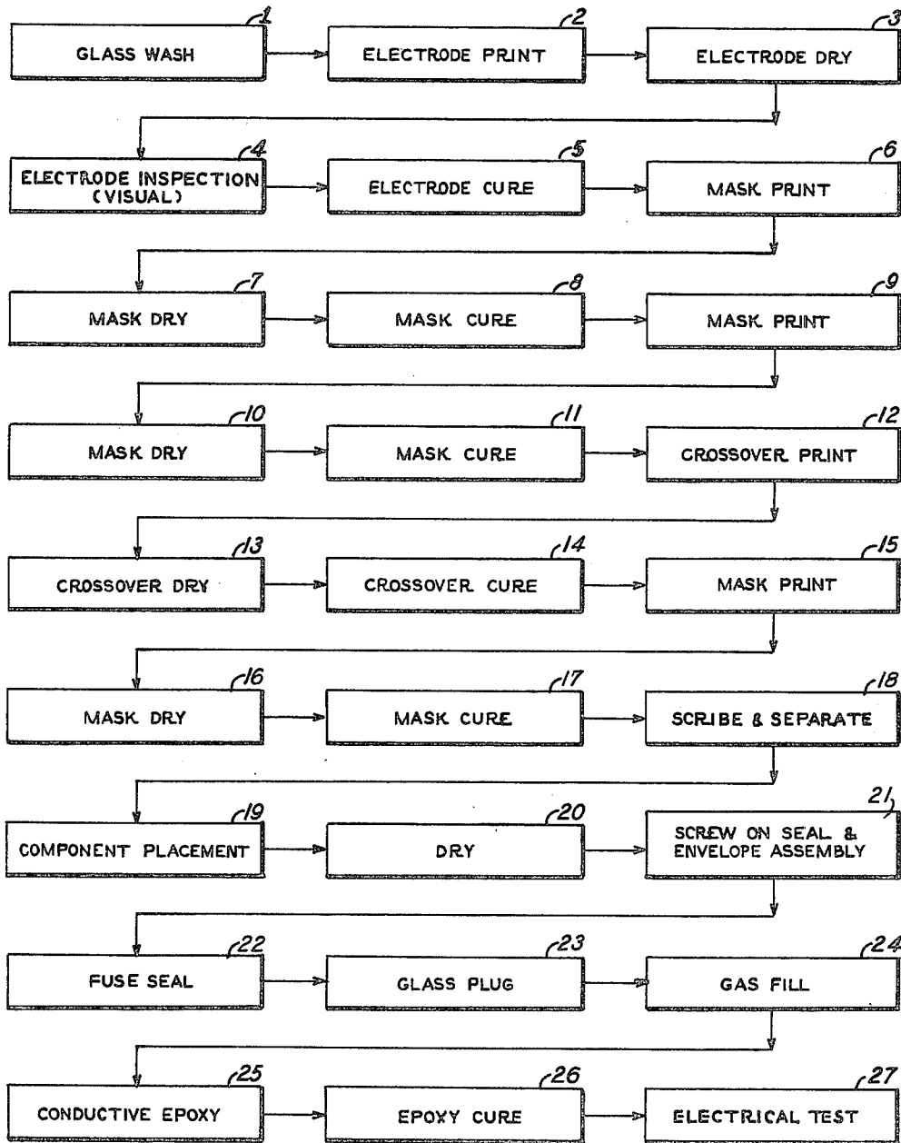
PROCESS FLOW CHART (NUMBERS REFER TO PROCESS STEPS)
