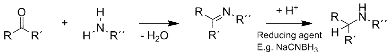
Scheme 4. Reductive amination
