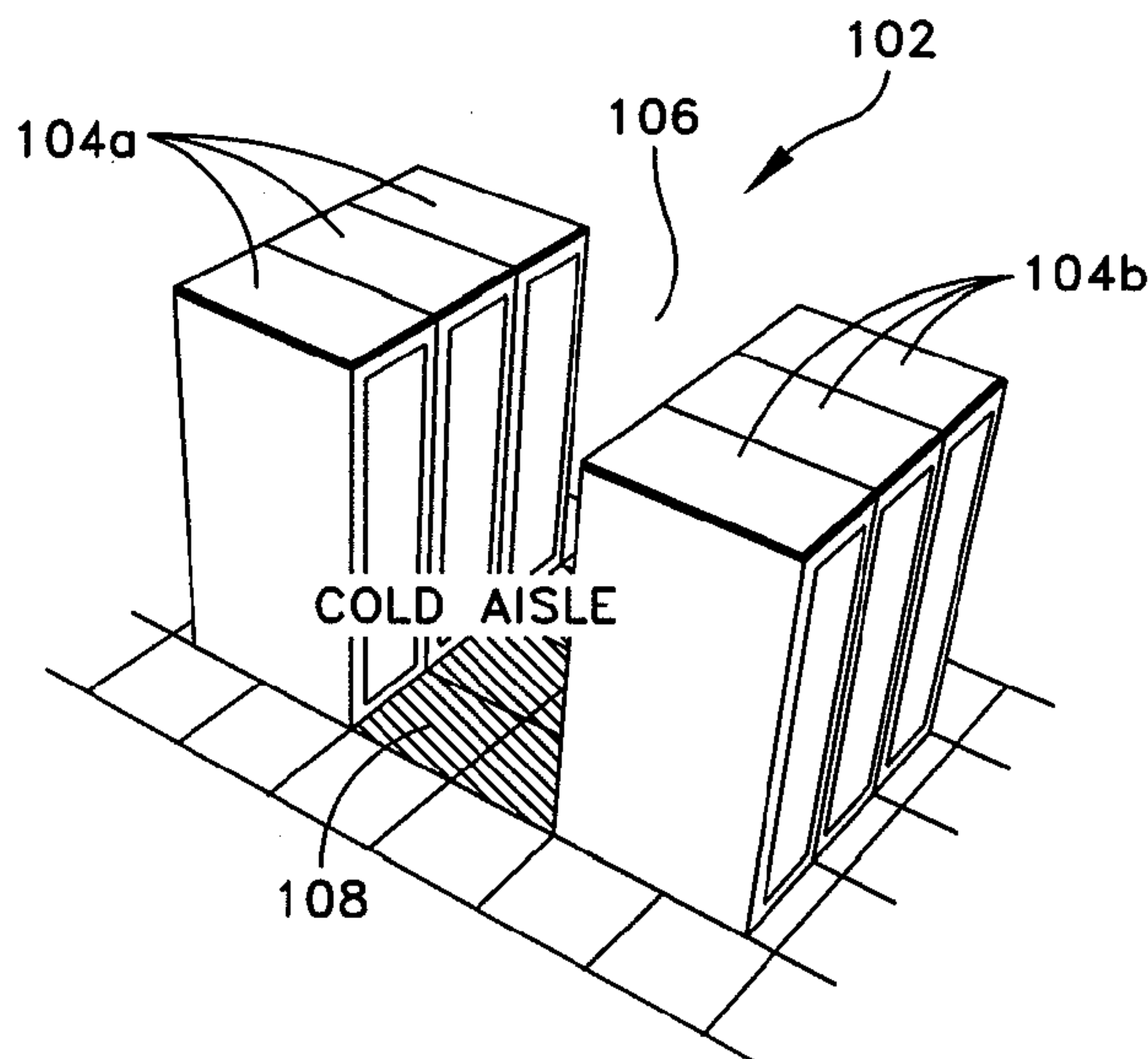
COLD-AISLE (RAISED-FLOOR) CLUSTER
