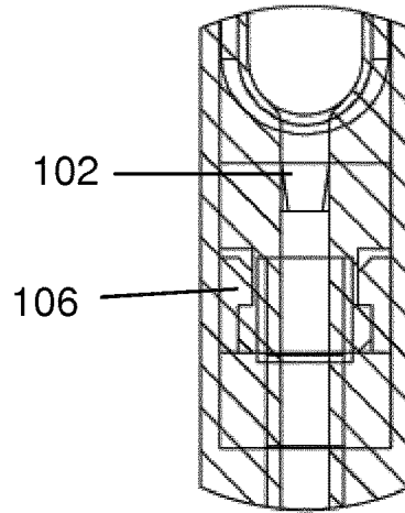
DETAIL C
