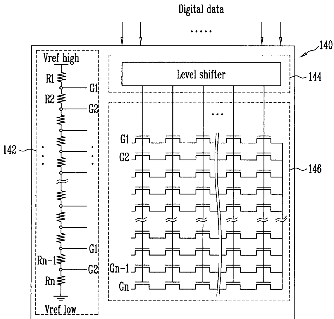
FIG. 2 (RELATED ART)
