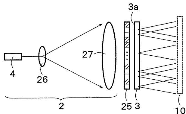
1 : ILLUMINATION DEVICE
