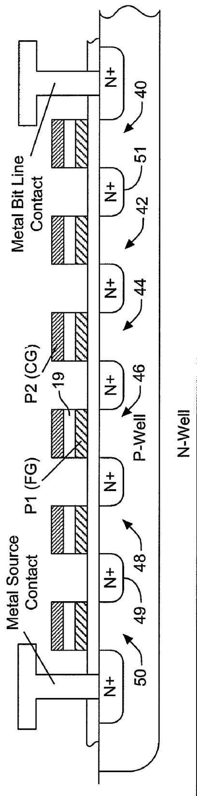
FIG. 2B (PRIOR ART) (Section A-A)
