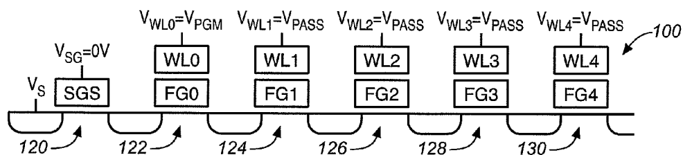
FIG. 6A (PRIOR ART)
