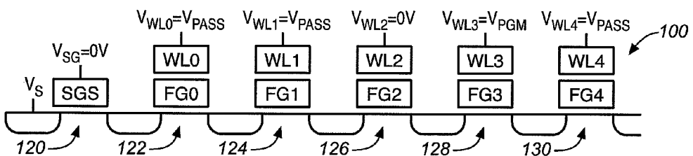
FIG. 6D (PRIOR ART)
