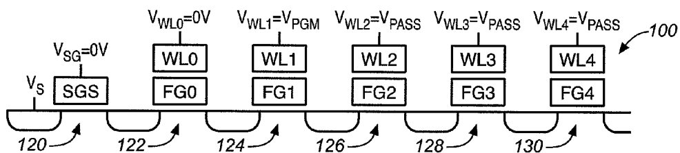
FIG. 6B (PRIOR ART)
