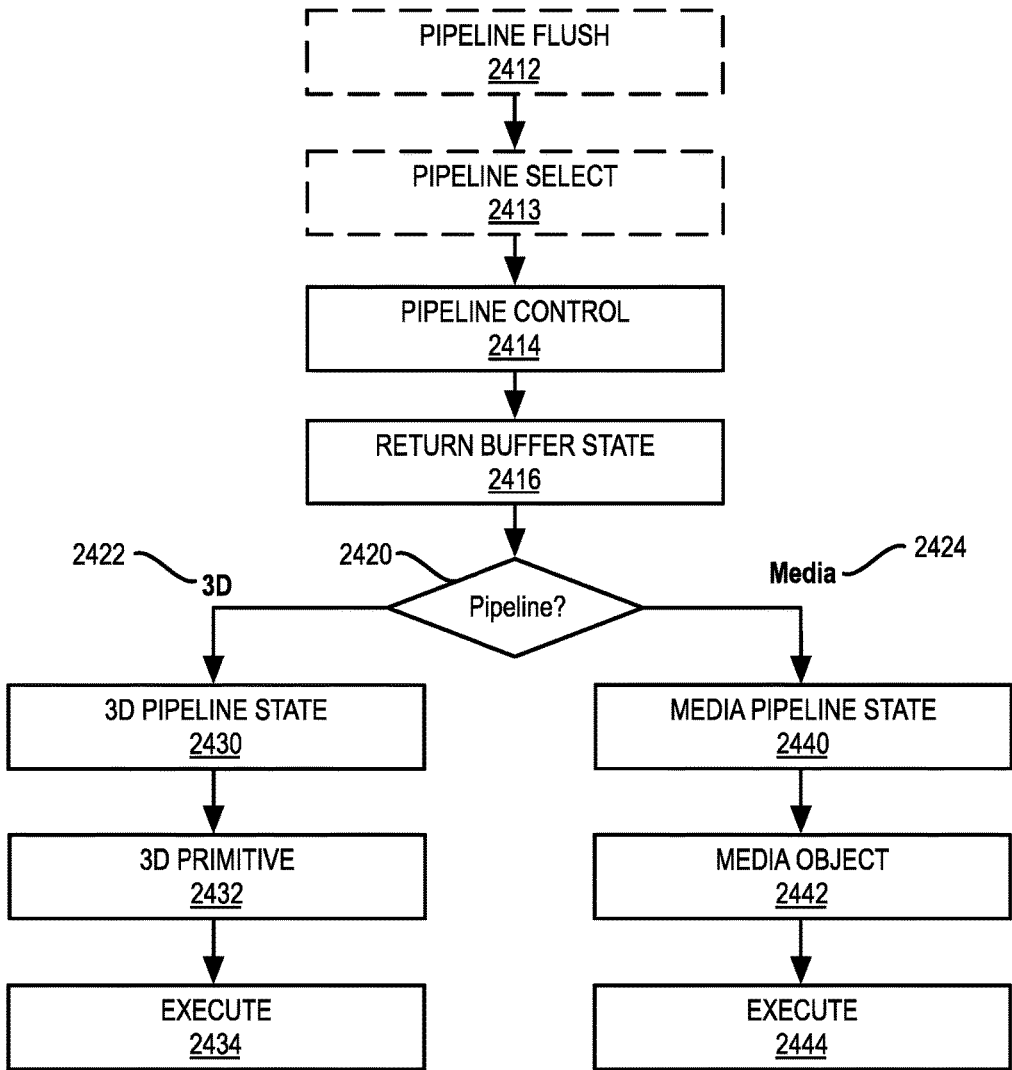
FIG. 24B GRAPHICS PROCESSOR COMMAND SEQUENCE 2410
