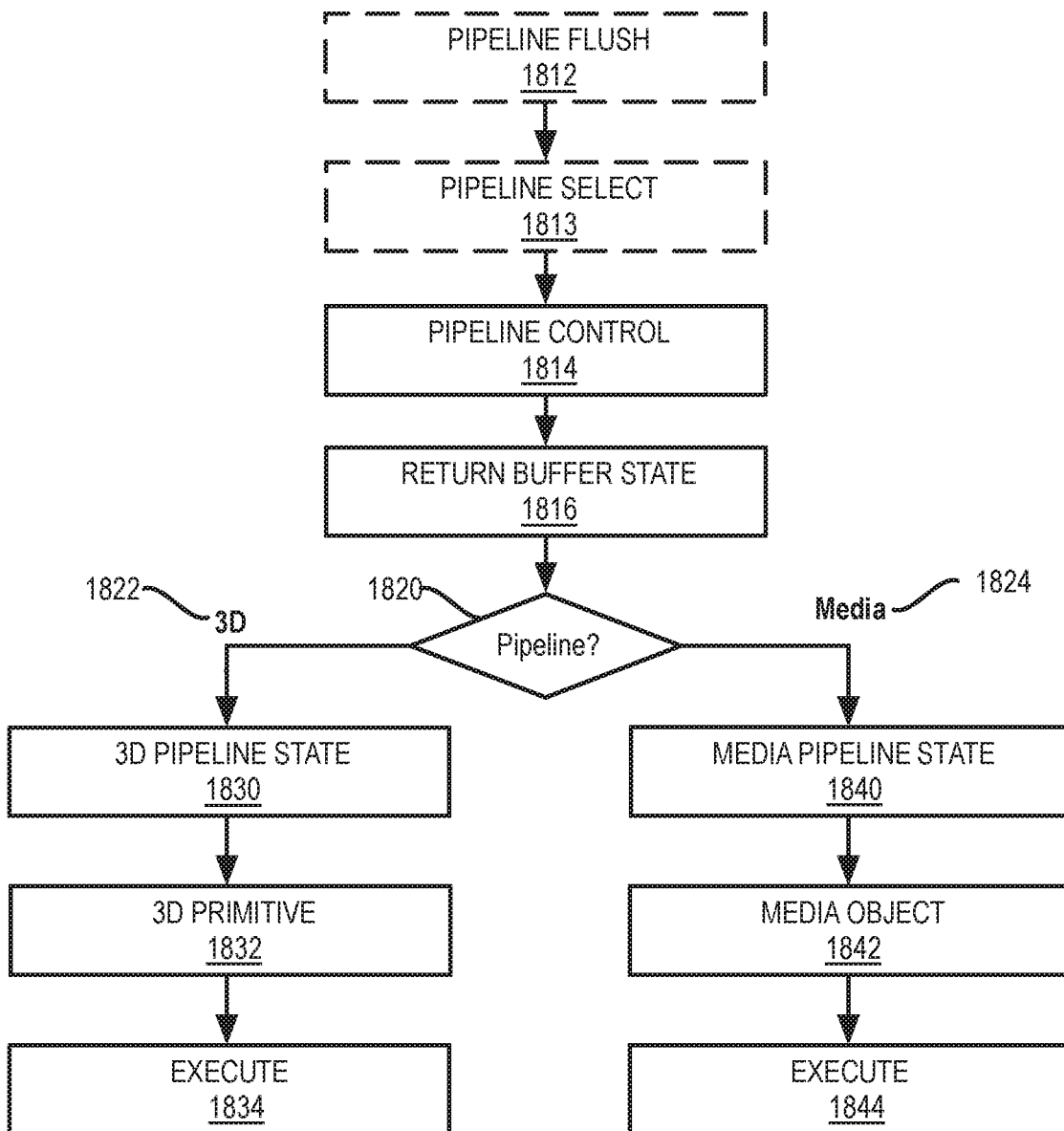
GRAPHICS PROCESSOR COMMAND SEQUENCE
