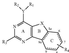
5a, 9a; 6, 7; and/or 8, 9-saturated or unsaturated
