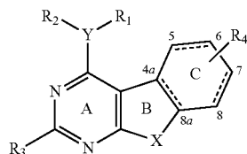
4a, 8a; 5, 6; and/or 7, 8-saturated or unsaturated
