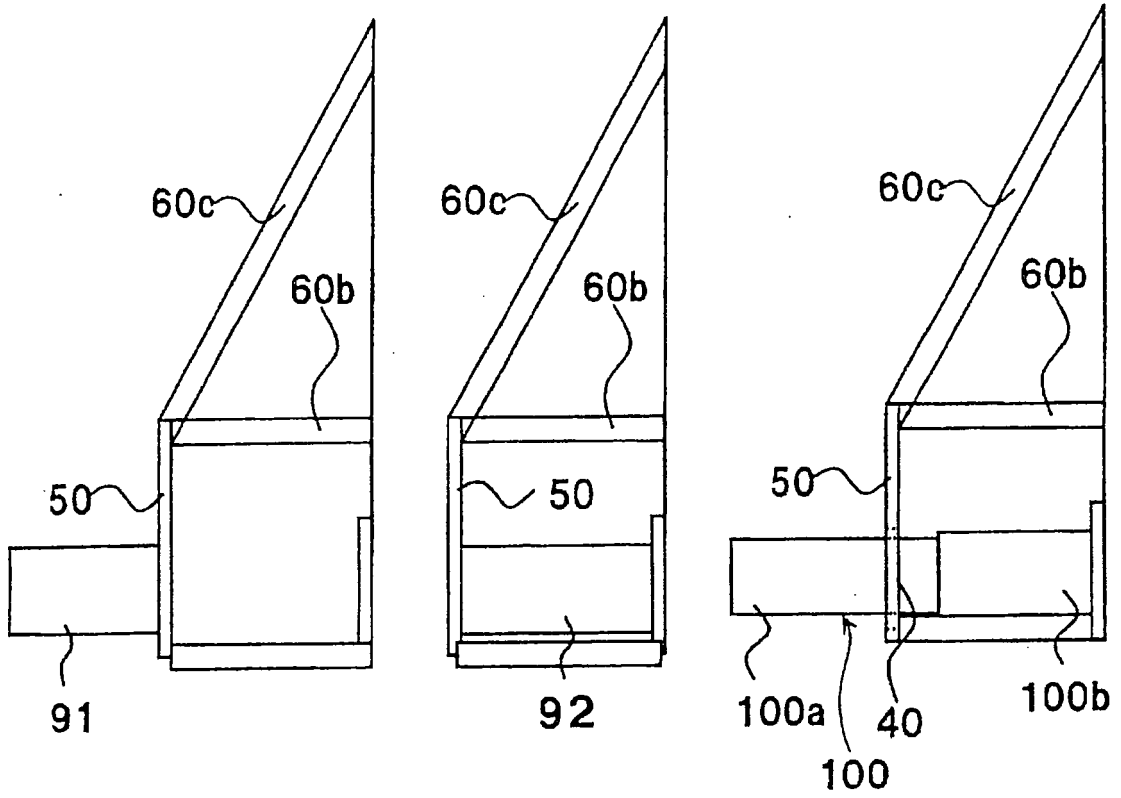
(b) CONVENTIONAL EMBODIMENT 2
