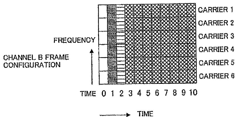
BASE STATION TRANSMIT SIGNAL FRAME CONFIGURATION
