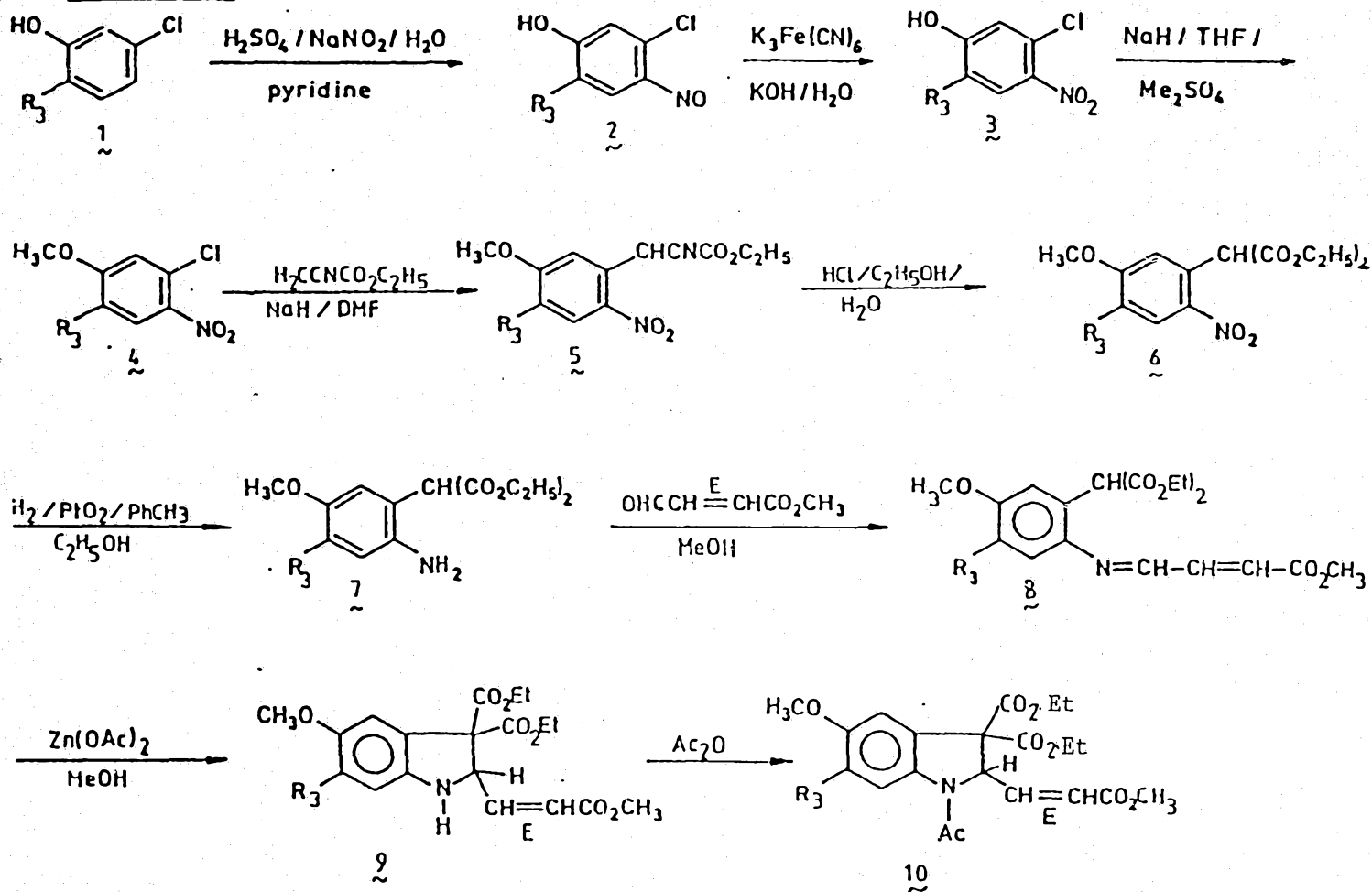
Scheme III
