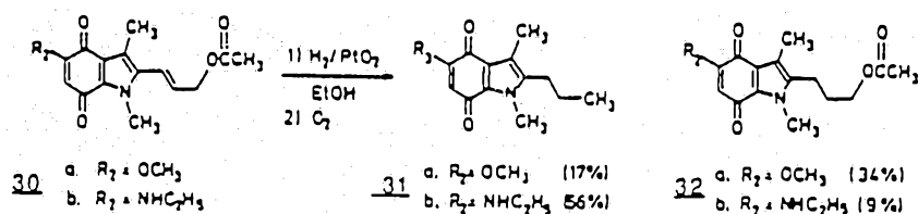
Scheme VIII
