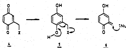
Scheme I B
