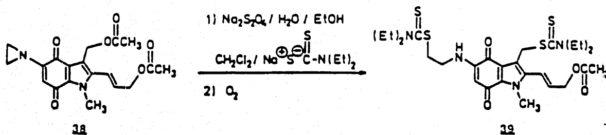
SCHEME XIII
