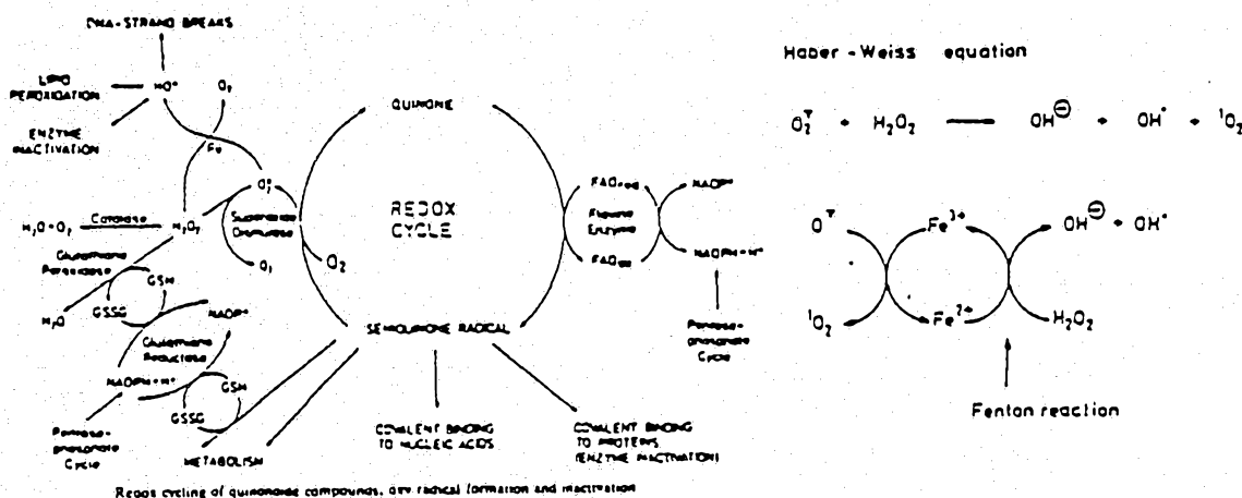
Scheme I A
