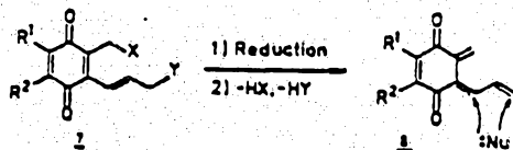
Scheme I C
