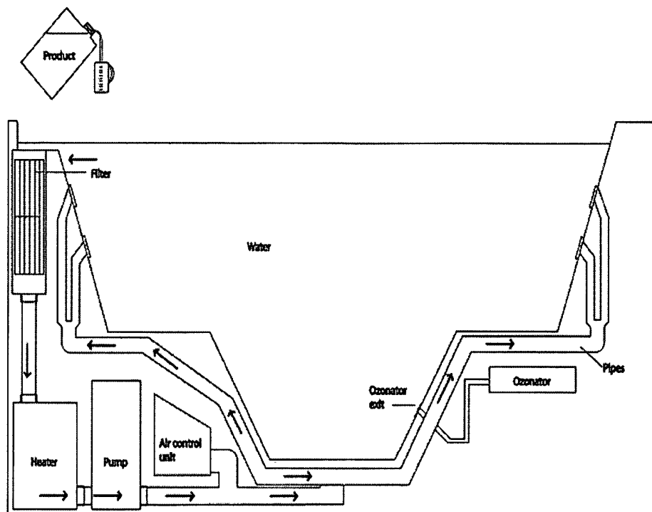
FIG 1. is a cross-sectional view of a hot tub. The product has to be poured onto the water surface once a week.
