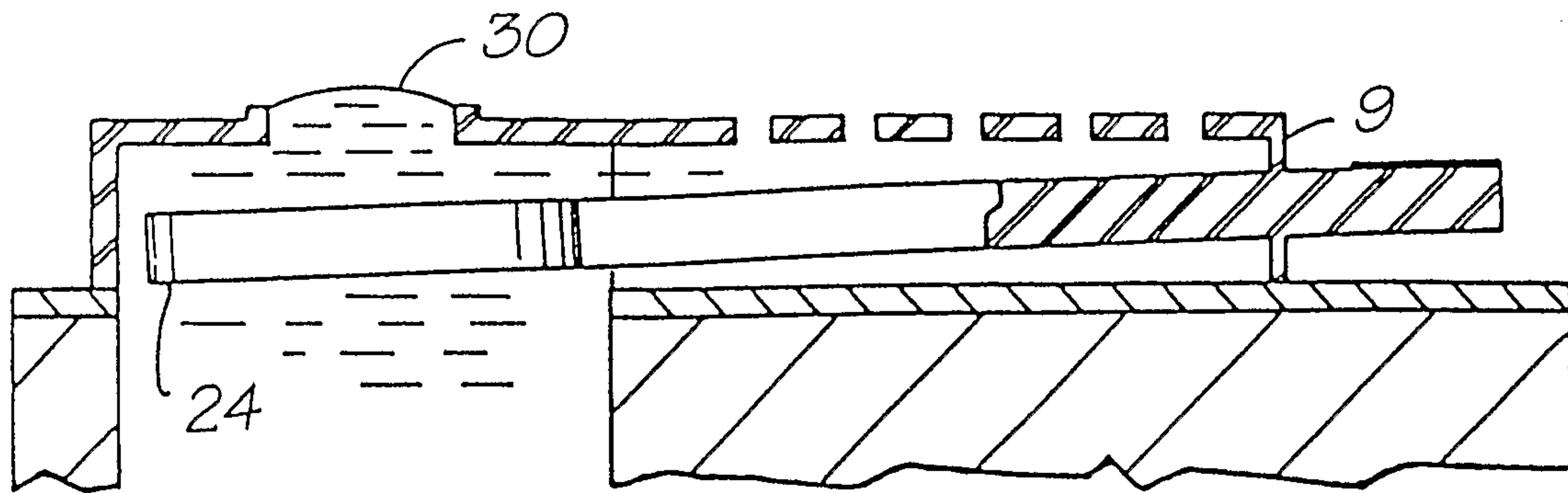
FIG. 3 (PRIOR ART)
