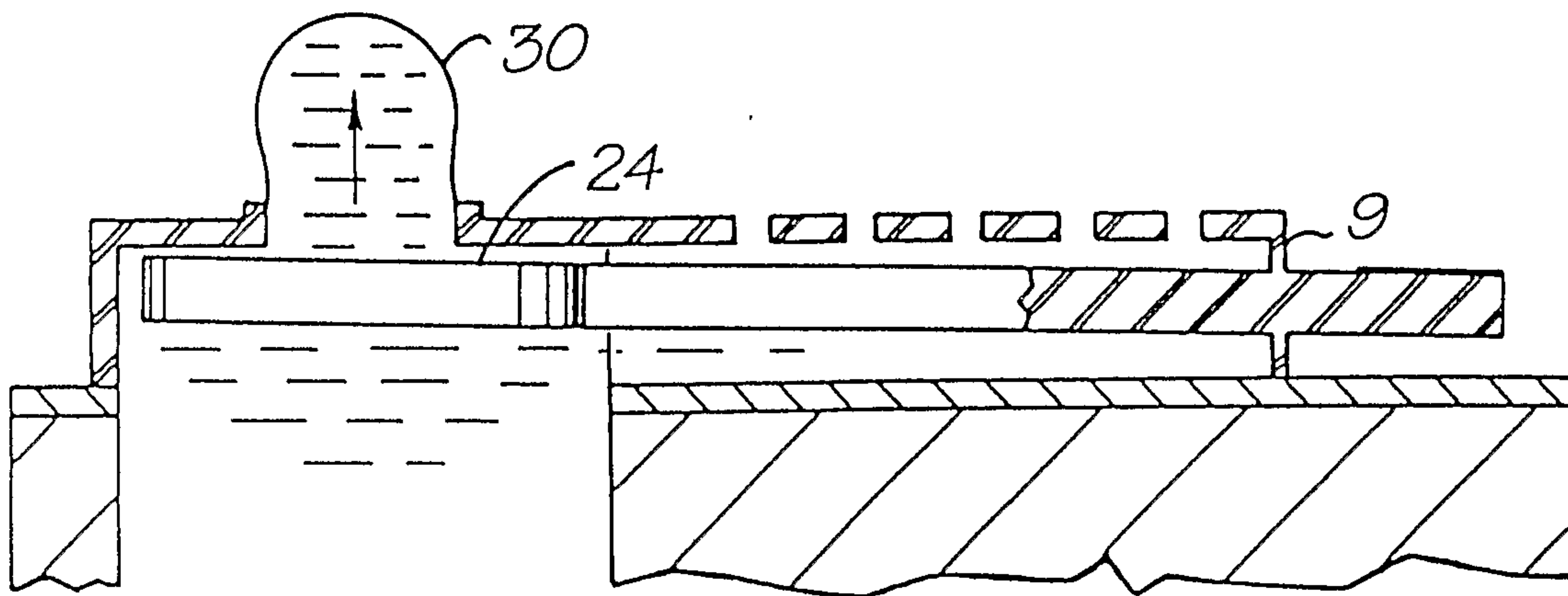
FIG. 4 (PRIOR ART)
