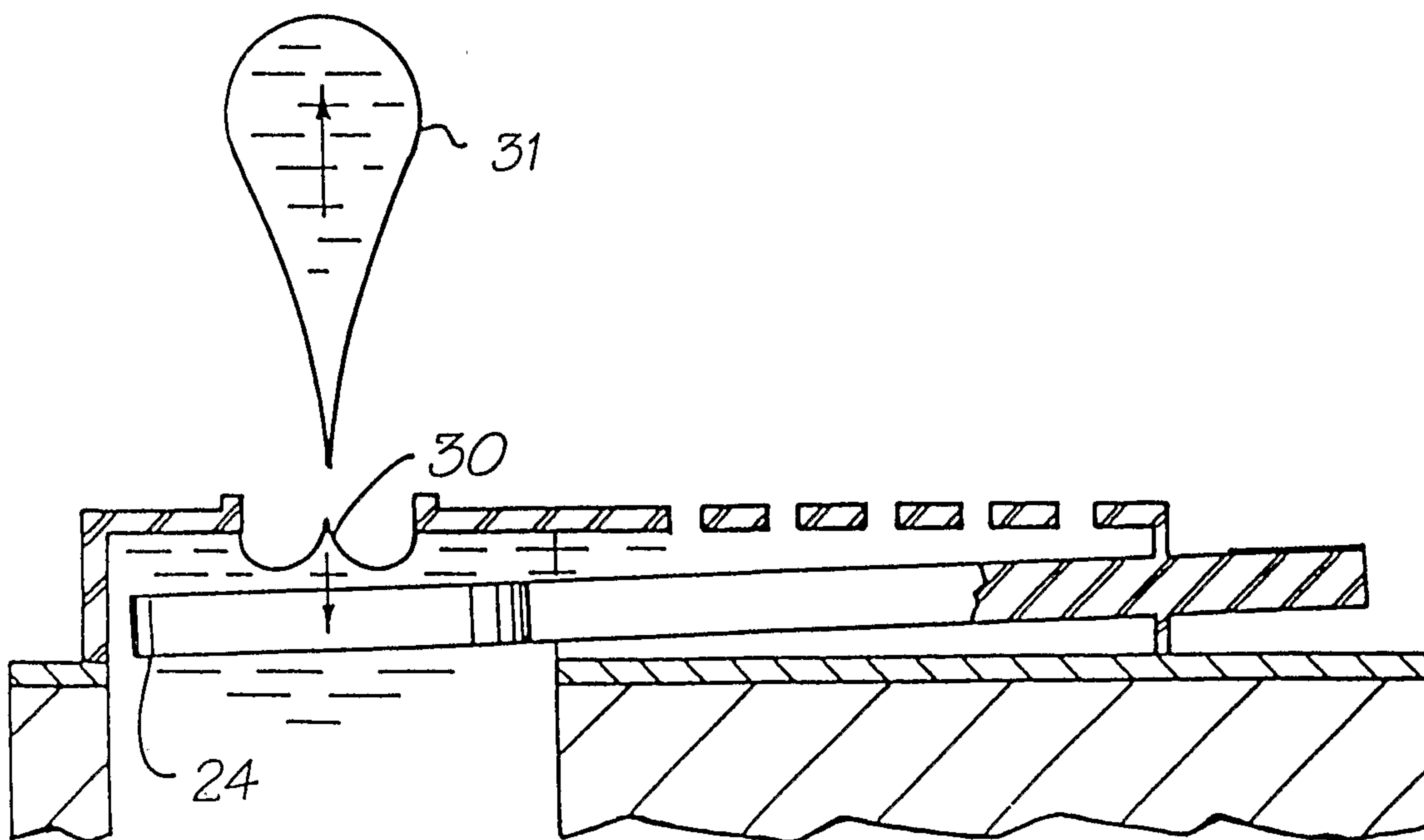
FIG. 5 (PRIOR ART)
