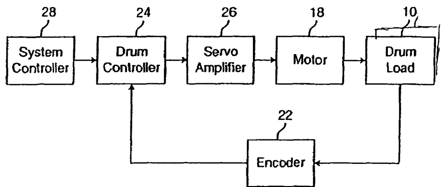
FIG. 1-B PRIOR ART
