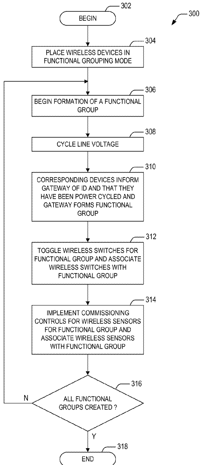
METHOD FOR CREATING FUNCTIONAL WIRELESS LIGHTING GROUPS
