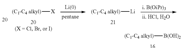
Scheme 3. Synthesis of Alkylboronic Ester 16
