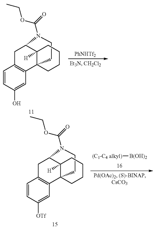
Scheme 2. Synthesis of a Compound of Formula I (R 1 is —(C 1 -C 4 )alkyl)
