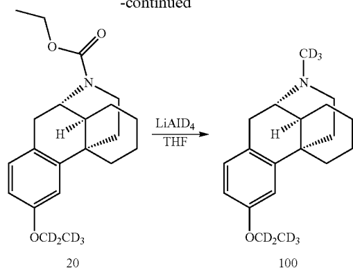
Synthesis of (+)-3-methoxy-17-methyl-(9 \alpha ,13 \alpha ,14 \alpha )-morphinan (free base, 8)
