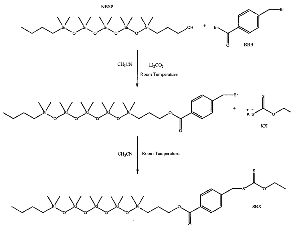
Reaction Scheme III
