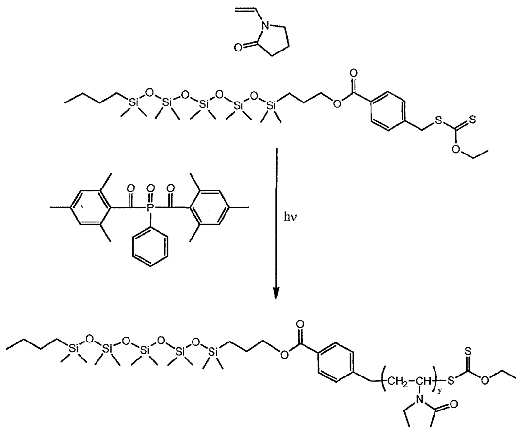
Reference Reaction Scheme IV
