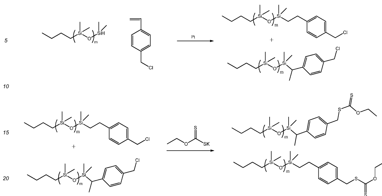
Reaction Scheme II
