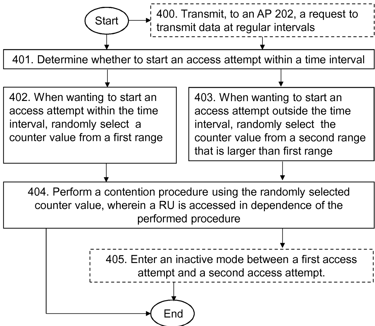
Figure 4 Method performed by communications device 204
