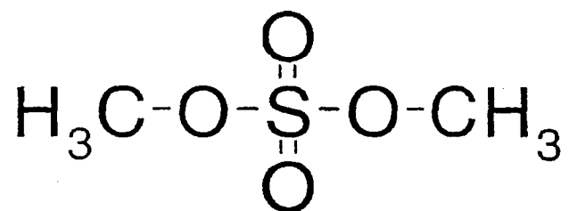
Structure 1: Dimethyl Sulphate
