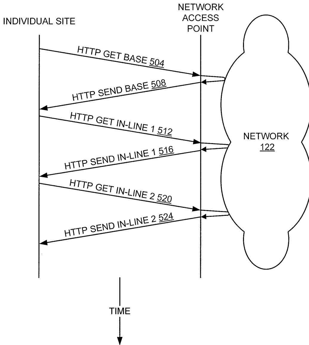
Fig. 5 Prior Art
