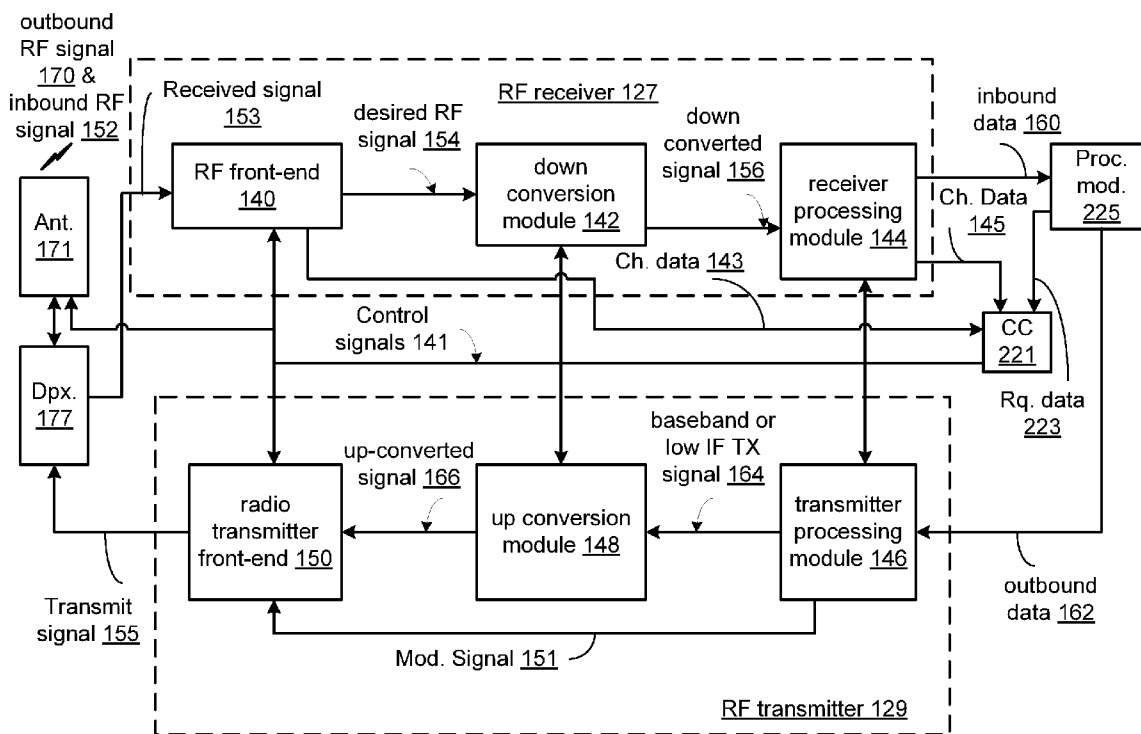
RF transceiver 123
