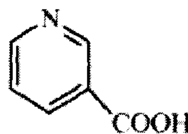
nicotinic acid
