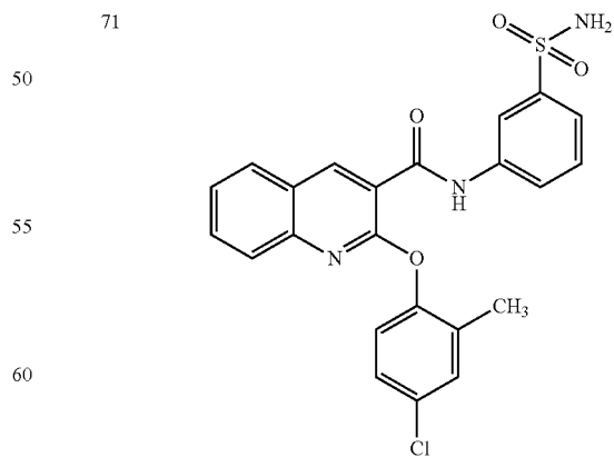
2-(4-chloro-2-methylphenoxy)-N-(3-sulfamoylphenyl)quinoline-3-carboxamide
