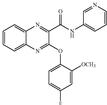
3-(4-fluoro-2-methoxyphenoxy)-N-(pyridin-3-yl)quinoxaline-2-carboxamide
