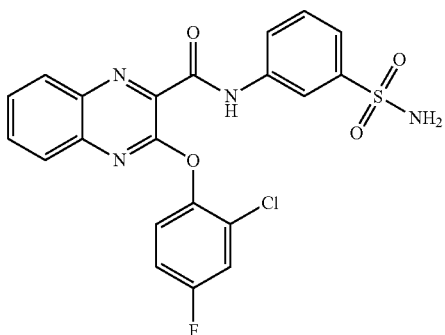
3-(2-chloro-4-fluorophenoxy)-N-(3-sulfamoylphenyl)quinoxaline-2-carboxamide
