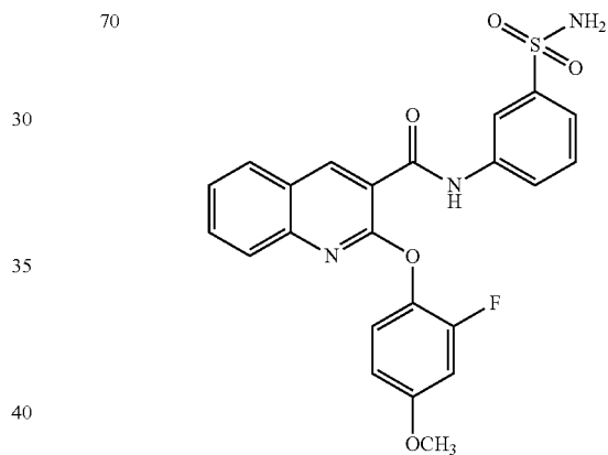
2-(2-fluoro-4-methoxyphenoxy)-N-(3-sulfamoylphenyl)quinoline-3-carboxamide
