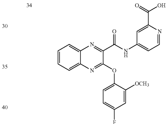
4-(3-(4-fluoro-2-methoxyphenoxy)quinoxaline-2-carboxamido)picolinic acid
