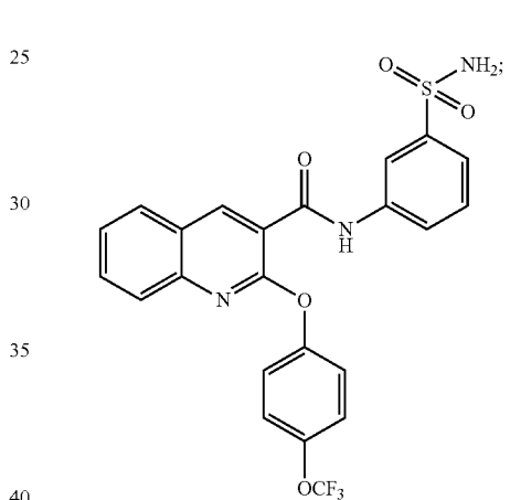
N-(3-sulfamoylphenyl)-2-(4-(trifluoromethoxy)phenoxy)quinoline-3-carboxamide
