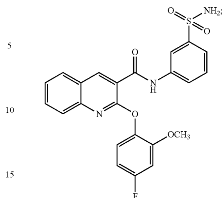
2-(4-fluoro-2-methoxyphenoxy)-N-(3-sulfamoylphenyl)quinoline-3-carboxamide
