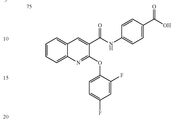
4-(2-(2,4-difluorophenoxy)quinoline-3-carboxamido)benzoic acid
