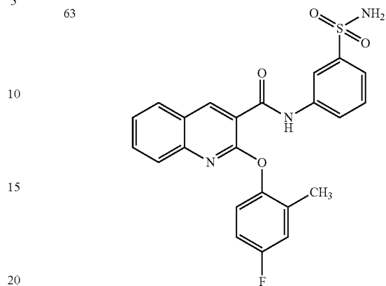
2-(4-fluoro-2-methylphenoxy)-N-(3-sulfamoylphenyl)quinoline-3-carboxamide
