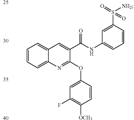
2-(3-fluoro-4-methoxyphenoxy)-N-(3-sulfamoylphenyl)quinoline-3-carboxamide
