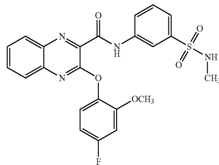
3-(4-fluoro-2-methoxyphenoxy)-N-(N-methylsulfamoylphenyl)quinoxaline-2-carboxamide
