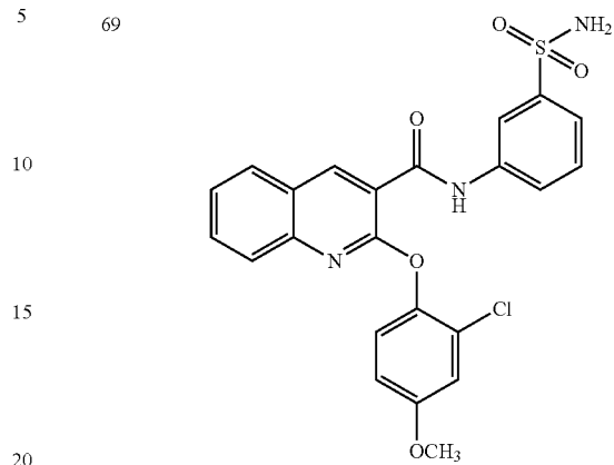
2-(2-chloro-4-methoxyphenoxy)-N-(3-sulfamoylphenyl)quinoline-3-carboxamide
