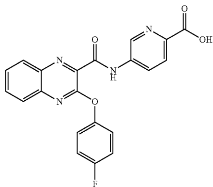
5-(3-(4-fluorophenoxy)quinoxaline-2-carboxamido)picolinic acid
