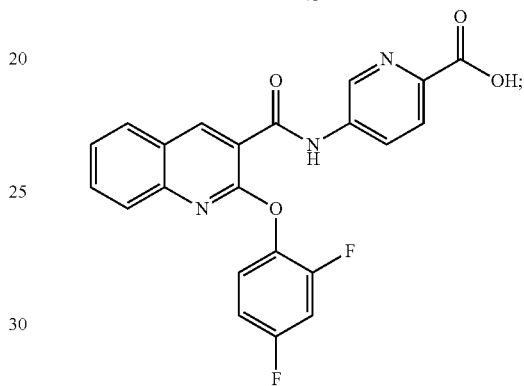
5-(2-(2,4-difluorophenoxy)quinoline-3-carboxamido)picolinic acid
