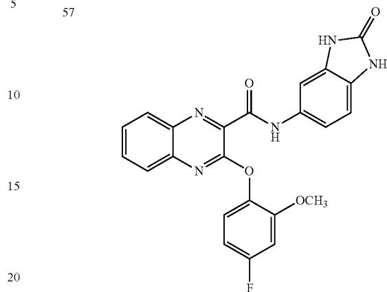
3-(4-fluoro-2-methoxyphenoxy)-N-(2-oxo-2,3-dihydro-1H-benzo[d]imidazol-5-yl)quinoxaline-2-carboxamide
