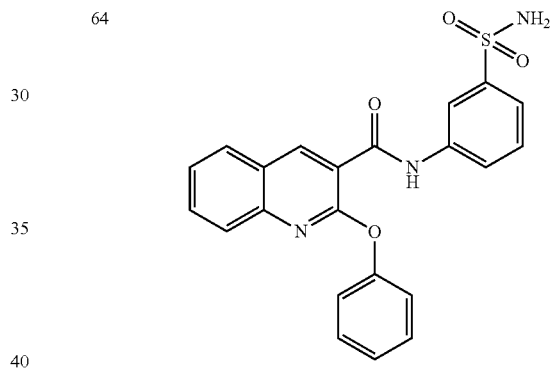
2-phenoxy-N-(3-sulfamoylphenyl)quinoline-3-carboxamide
