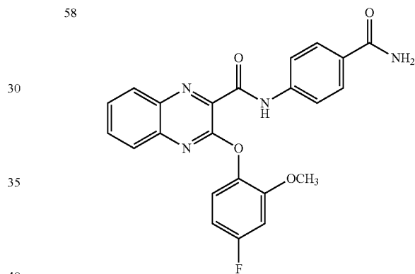
N-(4-carbamoylphenyl)-3-(4-fluoro-2-methoxyphenoxy)quinoxaline-2-carboxamide
