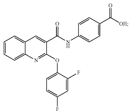
4-(2-(2,4-difluorophenoxy)quinoline-3-carboxamido)benzoic acid
