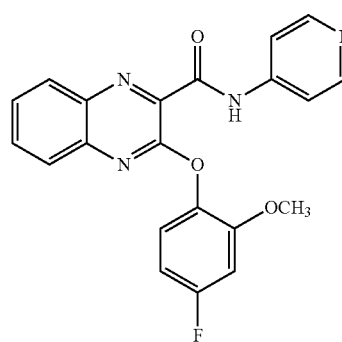
3-(4-fluoro-2-methoxyphenoxy)-N-(pyridin-4-yl)quinoxaline-2-carboxamide
