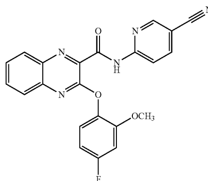
N-(5-cyanopyridin-2-yl)-3-(4-fluoro-2-methoxyphenoxy)quinoxaline-2-carboxamide
