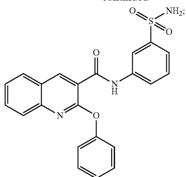
2-phenoxy-N-(3-sulfamoylphenyl)quinoline-3-carboxamide
