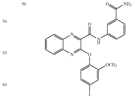
N-(3-carbamoylphenyl)-3-(4-fluoro-2-methoxyphenoxy)quinoxaline-2-carboxamide
