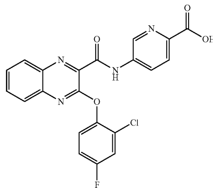
5-(3-(2-chloro-4-fluorophenoxy)quinoxaline-2-carboxamido)picolinic acid
