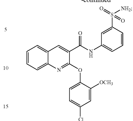
2-(4-chloro-2-methoxyphenoxy)-N-(3-sulfamoylphenyl)quinoline-3-carboxamide
