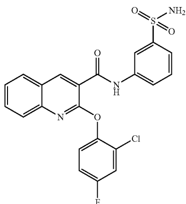
2-(2-chloro-4-fluorophenoxy)-N-(3-sulfamoylphenyl)quinoline-3-carboxamide
