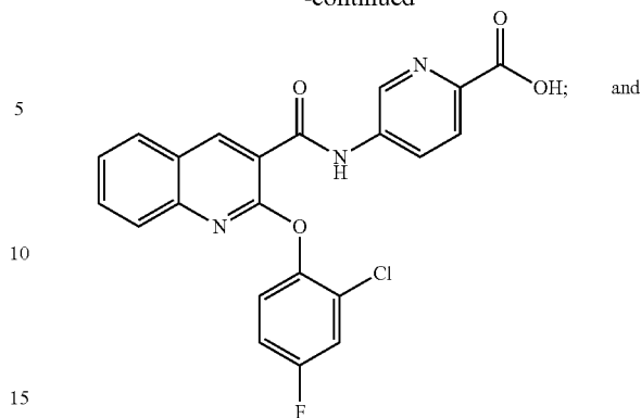
5-(2-(2-chloro-4-fluorophenoxy)quinoline-3-carboxamido)picolinic acid
