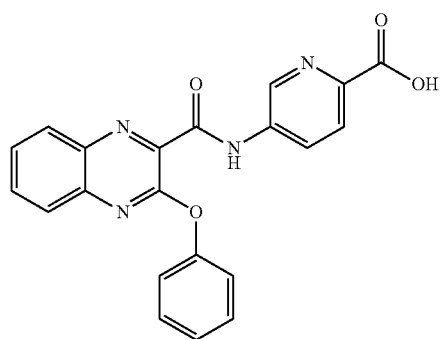
5-(3-phenoxyquinoxaline-2-carboxamido)picolinic acid
