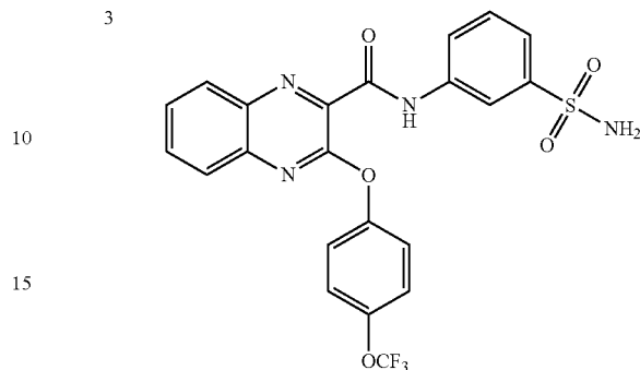
N-(3-sulfamoylphenyl)-3-(4-(trifluoromethoxy)phenoxy)quinoxaline-2-carboxamide
