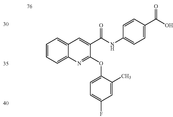
4-(2-(4-fluoro-2-methylphenoxy)quinoline-3-carboxamido)benzoic acid
