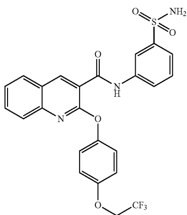
N-(3-sulfamoylphenyl)-2-(4-(2,2,2-trifluoroethoxy)phenoxy)quinoline-3-carboxamide
