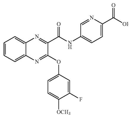
5-(3-(3-fluoro-4-methoxyphenoxy)quinoxaline-2-carboxamido)picolinic acid
