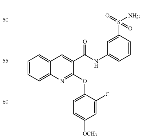
2-(2-chloro-4-methoxyphenoxy)-N-(3-sulfamoylphenyl)quinoline-3-carboxamide
