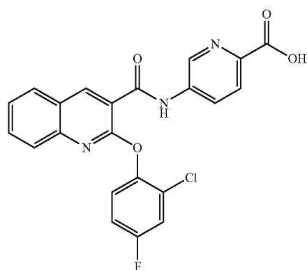
5-(2-(2-chloro-4-fluorophenoxy)quinoline-3-carboxamido)picolinic acid
