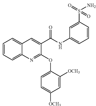
2-(2,4-dimethoxyphenoxy)-N-(3-sulfamoylphenyl)quinoline-3-carboxamide
