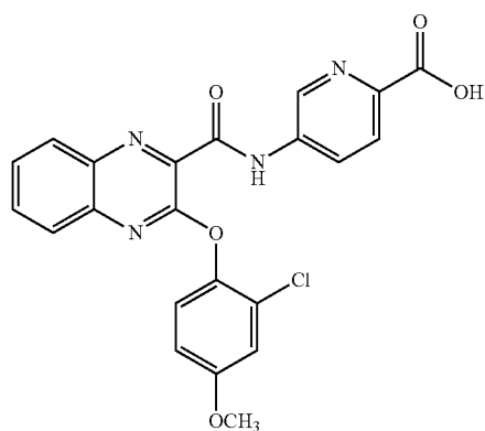
5-(3-(2-chloro-4-methoxyphenoxy)quinoxaline-2-carboxamido)picolinic acid
