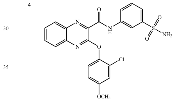
3-(2-chloro-4-methoxyphenoxy)-N-(3-sulfamoylphenyl)quinoxaline-2-carboxamide
