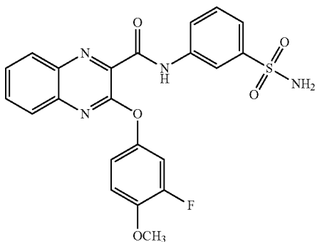
3-(3-fluoro-4-methoxyphenoxy)-N-(3-sulfamoylphenyl)quinoxaline-2-carboxamide
