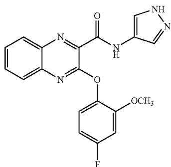
3-(4-fluoro-2-methoxyphenoxy)-N-(1H-pyrazol-4-yl)quinoxaline-2-carboxamide
