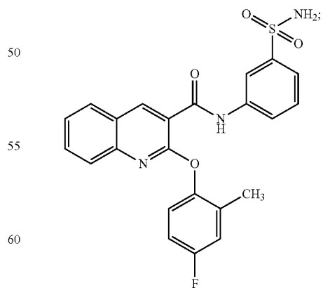
2-(4-fluoro-2-methylphenoxy)-N-(3-sulfamoylphenyl)quinoline-3-carboxamide
