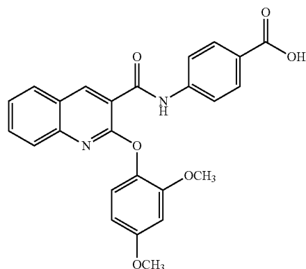
4-(2-(2,4-dimethoxyphenoxy)quinoline-3-carboxamido)benzoic acid
