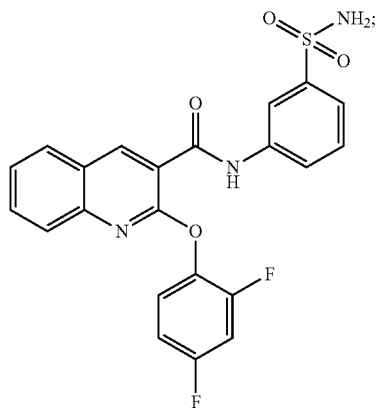
2-(2,4-difluorophenoxy)-N-(3-sulfamoylphenyl)quinoline-3-carboxamide
