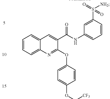
N-(3-sulfamoylphenyl)-2-(4-(2,2,2-trifluoroethoxy)phenoxy)quinoline-3-carboxamide
