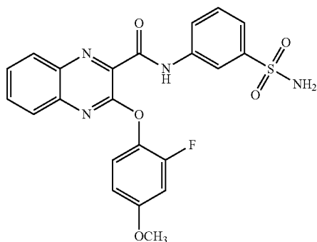
3-(2-fluoro-4-methoxyphenoxy)-N-(3-sulfamoylphenyl)quinoxaline-2-carboxamide
