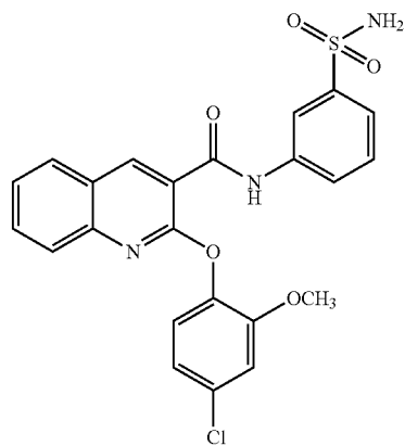
2-(4-chloro-2-methoxyphenoxy)-N-(3-sulfamoylphenyl)quinoline-3-carboxamide
