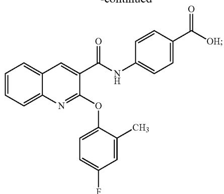
4-(2-(4-fluoro-2-methylphenoxy)quinoline-3-carboxamido)benzoic acid
