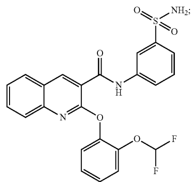
2-(2-(difluoromethoxy)phenoxy)-N-(3-sulfamoylphenyl)quinoline-3-carboxamide
