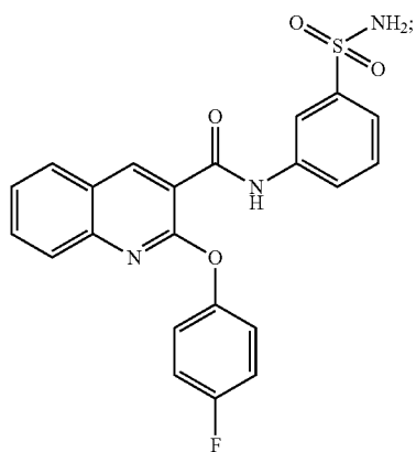
2-(4-fluorophenoxy)-N-(3-sulfamoylphenyl)quinoline-3-carboxamide
