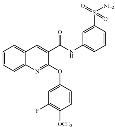
2-(3-fluoro-4-methoxyphenoxy)-N-(3-sulfamoylphenyl)quinoline-3-carboxamide
