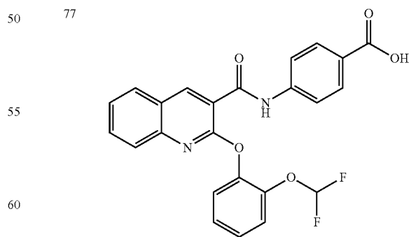
4-(2-(2-(difluoromethoxy)phenoxy)quinoline-3-carboxamido)benzoic acid
