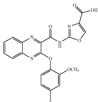
2-(3-(4-fluoro-2-methoxyphenoxy)quinoxaline-2-carboxamido)oxazole-4-carboxylic acid
