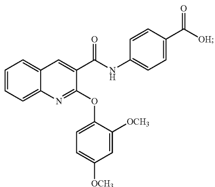
4-(2-(2,4-dimethoxyphenoxy)quinoline-3-carboxamido)benzoic acid
