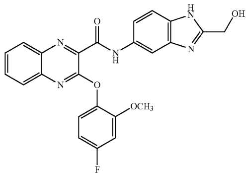
3-(4-fluoro-2-methoxyphenoxy)-N-(2-(hydroxymethyl)-1H-benzodimidazol-5-yl)quinoxaline-2-carboxamide
