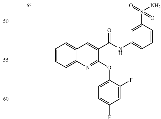
2-(2,4-difluorophenoxy)-N-(3-sulfamoylphenyl)quinoline-3-carboxamide
