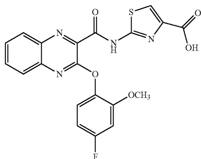
2-(3-(4-fluoro-2-methoxyphenoxy)quinoxaline-2-carboxamido)thiazole-4-carboxylic acid
