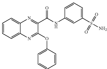
3-phenoxy-N-(3-sulfamoylphenyl)quinoxaline-2-carboxamide
