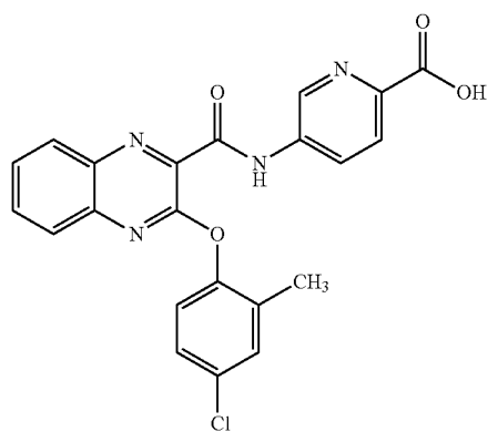
5-(3-(4-chloro-2-methylphenoxy)quinoxaline-2-carboxamido)picolinic acid
