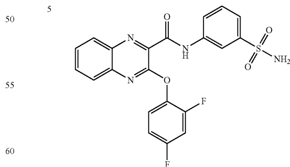
3-(2,4-difluorophenoxy)-N-(3-sulfamoylphenyl)quinoxaline-2-carboxamide
