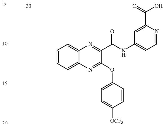
4-(3-(4-(trifluoromethoxy)phenoxy)quinoxaline-2-carboxamido)picolinic acid
