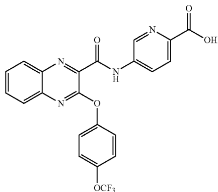
5-(3-(4-(trifluoromethoxy)phenoxy)quinoxaline-2-carboxamido)picolinic acid
