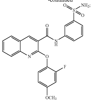
2-(2-fluoro-4-methoxyphenoxy)-N-(3-sulfamoylphenyl)quinoline-3-carboxamide
