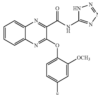
3-(4-fluoro-2-methoxyphenoxy)-N-(1H-tetrazol-5-yl)quinoxaline-2-carboxamide
