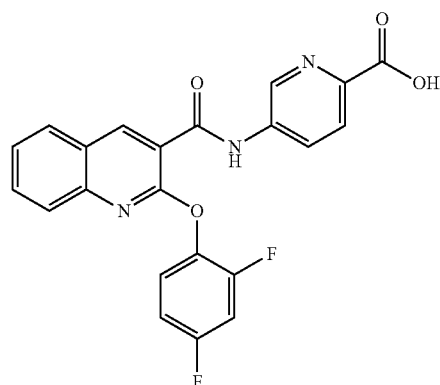
5-(2-(2,4-difluorophenoxy)quinoline-3-carboxamido)picolinic acid
