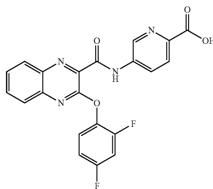
5-(3-(2,4-difluorophenoxy)quinoxaline-2-carboxamido)picolinic acid
