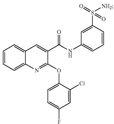
2-(2-chloro-4-fluorophenoxy)-N-(3-sulfamoylphenyl)quinoline-3-carboxamide
