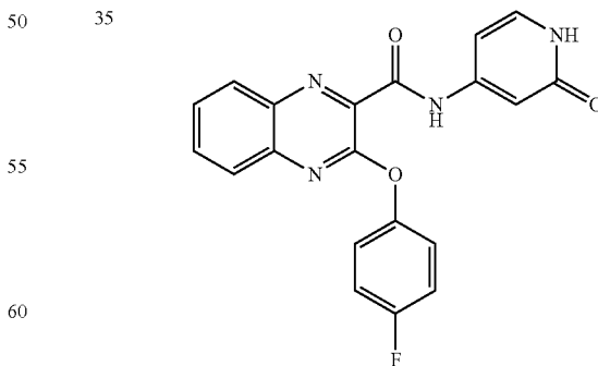
3-(4-fluorophenoxy)-N-(2-oxo-1,2-dihydropyridin-4-yl)quinoxaline-2-carboxamide
