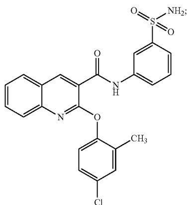
2-(4-chloro-2-methylphenoxy)-N-(3-sulfamoylphenyl)quinoline-3-carboxamide
