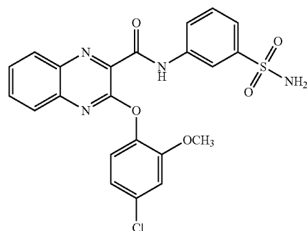
3-(4-chloro-2-methoxyphenoxy)-N-(3-sulfamoylphenyl)quinoxaline-2-carboxamide
