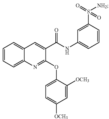
2-(2,4-dimethoxyphenoxy)-N-(3-sulfamoylphenyl)quinoline-3-carboxamide
