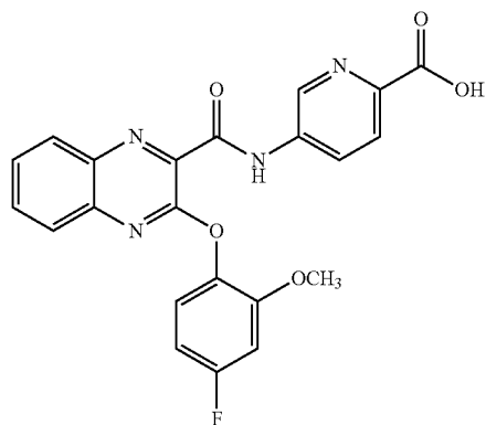
5-(3-(4-fluoro-2-methoxyphenoxy)quinoxaline-2-carboxamido)picolinic acid
