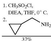
3-{[2-(5-Isoquinolin-4-yl-1H-indazol-3-yl)-1H-benzimidazol-4-ylmethyl]-amino}-2-methyl-propan-1-ol
