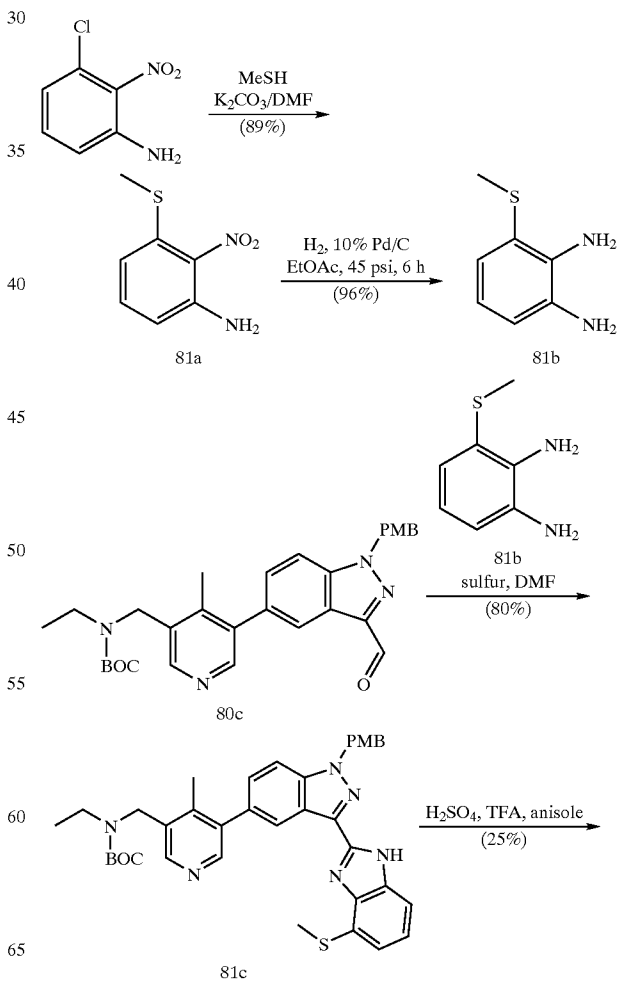
Ethyl-4-{methyl-5-[3-(4-methylsulfanyl-1H-benzimidazol-2-yl)-1H-indazol-5-yl]-pyridin-3-ylmethyl}-amine
