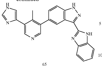
(a) Intermediate 65a—3-Bromo-4-methyl-5-1H-imidazol-4-yl-pyridine
