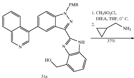
3-{[2-(5-Isoquinolin-4-yl-1H-indazol-3-yl)-1H-benzimidazol-4-ylmethyl]-amino}-2-methyl-propan-1-ol
