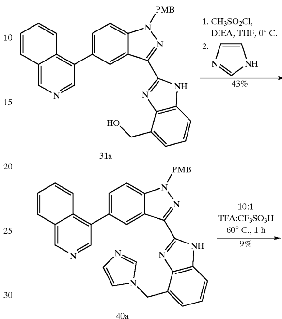
5 4-[3-(4-Imidazol-1-ylmethyl-1H-benzoimidazol-2-yl)-1H-indazol-5-yl]-isoquinoline
