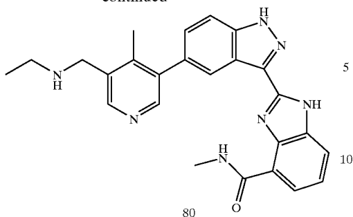
(a) Intermediate 80a—(5-Bromo-4-methyl-pyridin-3-ylmethyl)ethyl-amine
