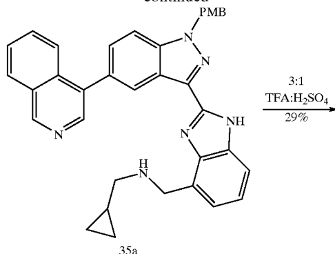
(a) Intermediate 35a—Cyclopropylmethyl-{2-[5-isoquinolin-4-yl-1H-indazol-3-yl]-1H-benzimidazol-4-ylmethyl}-amine
