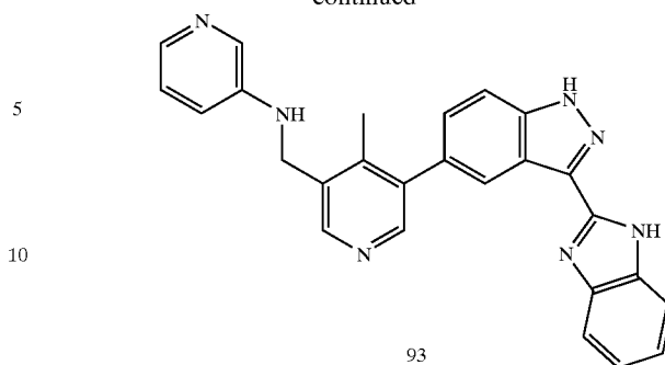
(a) Example 93—{5-[3-(1H-Benzoimidazol-2-yl)-1H-indazol-5-yl]-4-methyl-pyridin-3-ylmethyl}-pyridin-3-yl-amine
