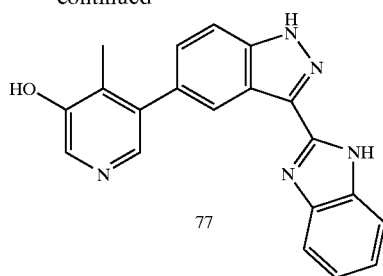
(a) Intermediate 77a—5-Bromo-4-methyl-pyridin-3-ol
