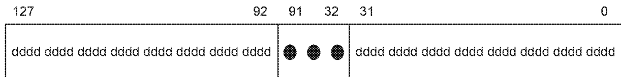
Unsigned Packed Doubleword Representation 348
