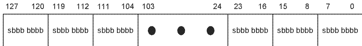
Signed Packed Byte Representation 345
