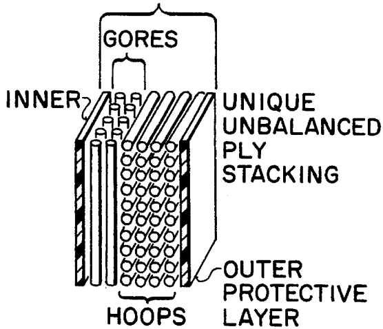
PRIMARY STRUCTURE
