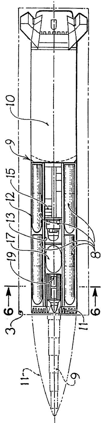
INFLATABLE NOSE FARING DESIGN
