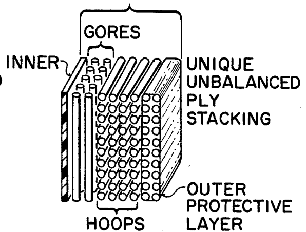
PRIMARY STRUCTURE
