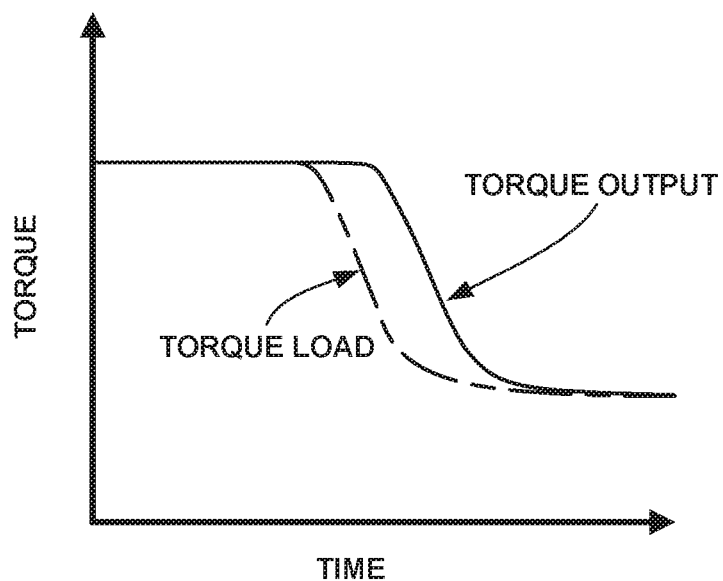
FIG. 8 (PRIOR ART)
