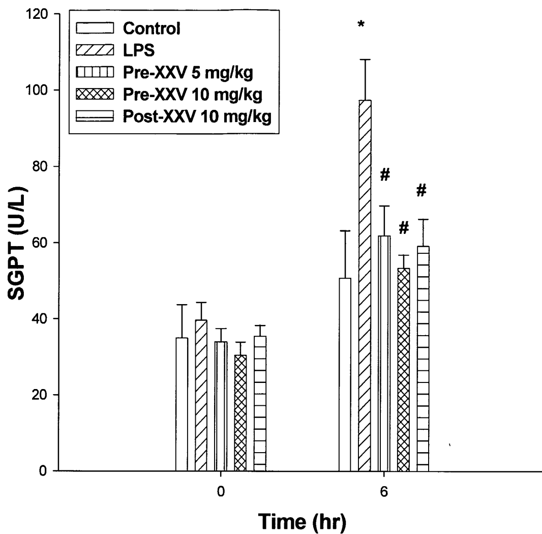
Figure 4. Effects of pre-treatment with XXV (5 mg/kg, i.v., n=9 and 10 mg/kg, i.v., n=10) and post-treatment XXV(10 mg/kg, i.v., n=6) on SGPT at 0 and 6 hr after LPS-treated rat (n=10). Data represent mean \pm S.E.M., * p < 0.05 : LPS vs. Control (n=4) and # p < 0.05 : XXV vs. LPS.
