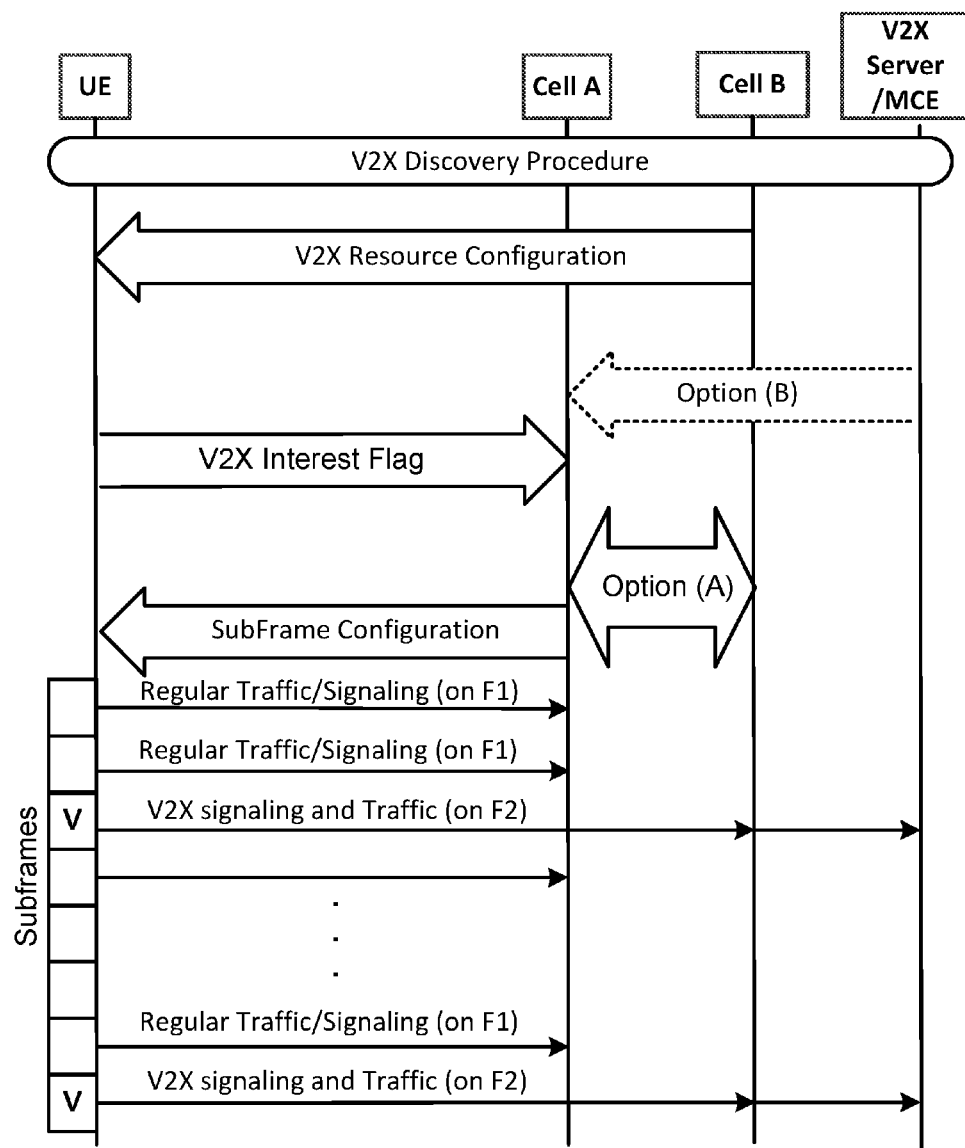
Time/Subframe Multiplexing Between F1 and F2
