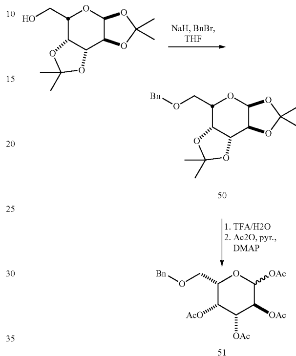
Scheme 13
