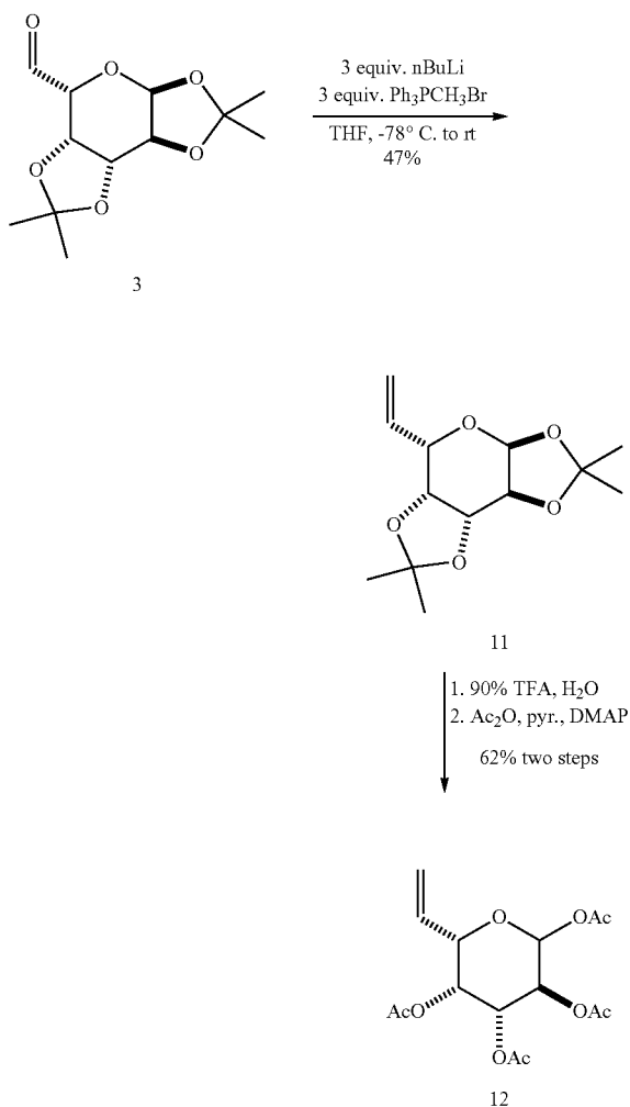
Scheme 4
