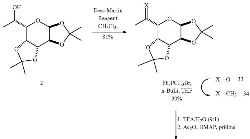
Scheme 8
