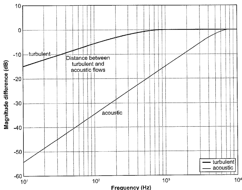
Ratio of diff and sum power spectrum for turbulent and acoustic propagation d= 0.02m
