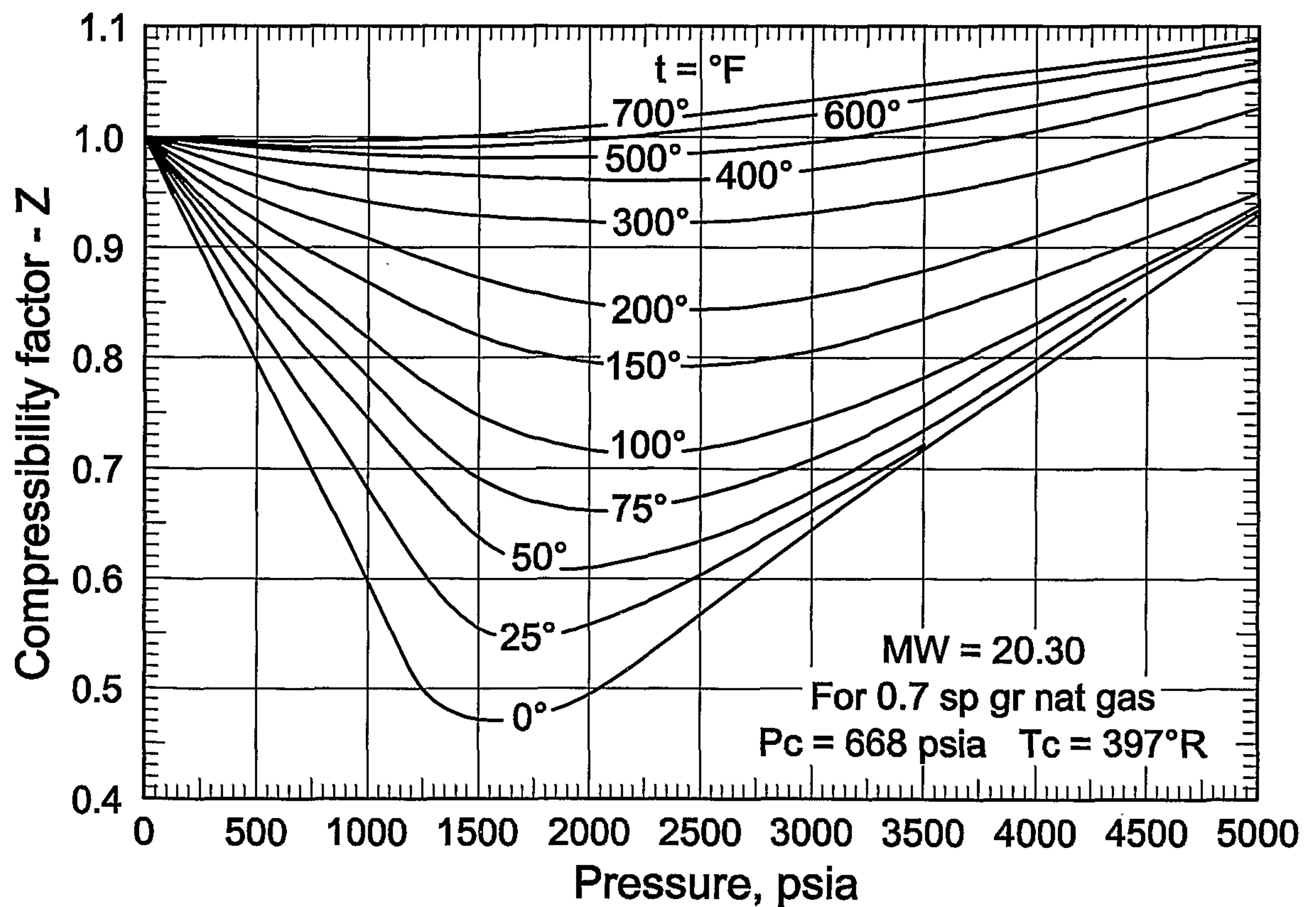
Fig. 2 Compressibility Factor for Natural Gas S. G. = 0.7
