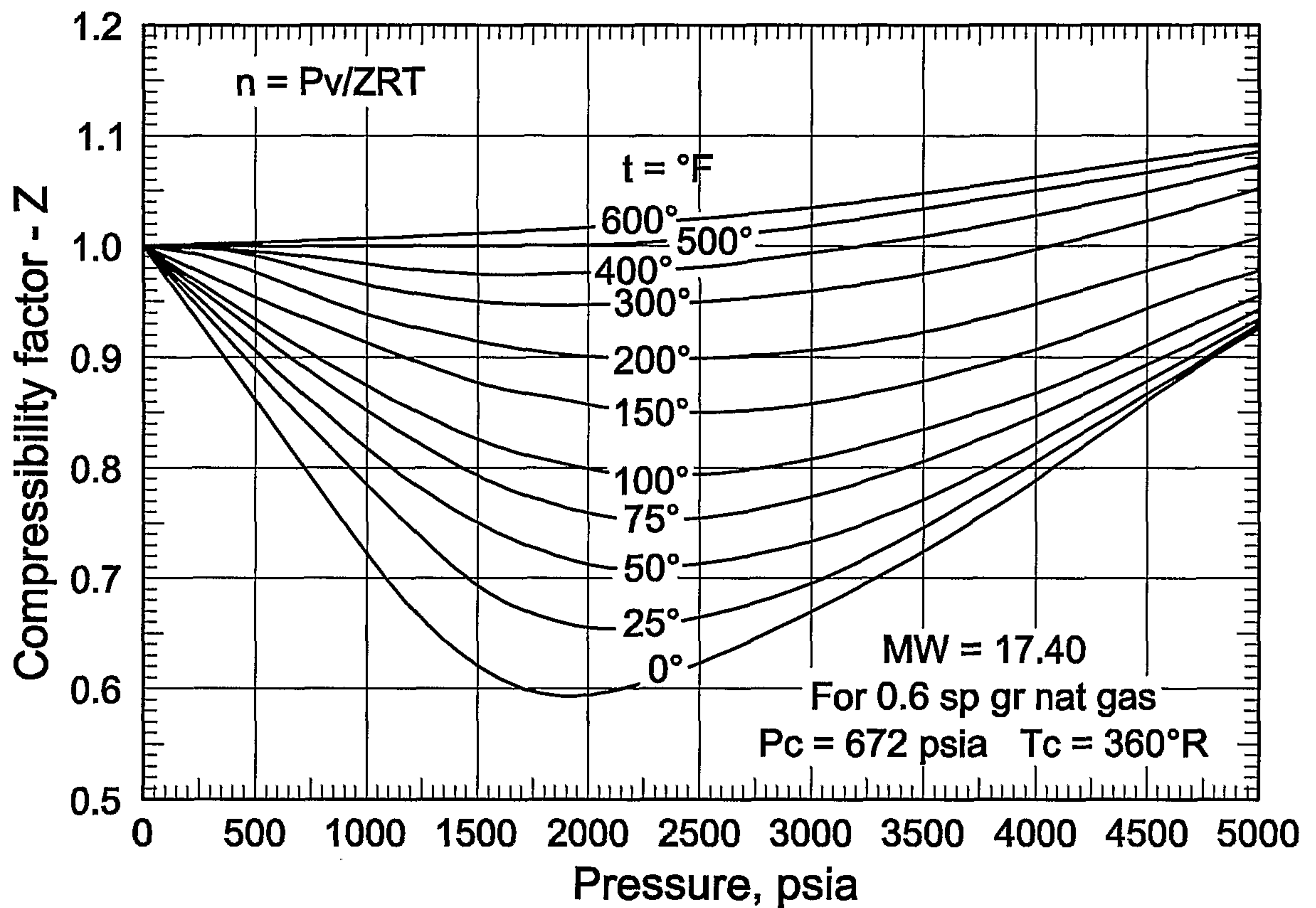
Fig. 1 Compressibility Factor for Natural Gas S. G. = 0.6
