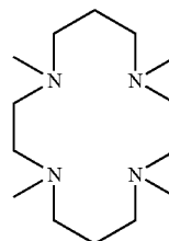
1,4,8,11-tetramethyl-1,4,8,11-tetraazacyclotetradecane
