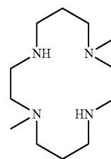
1,8-dimethyl-1,4,8,11-tetraazacyclotetradecane
