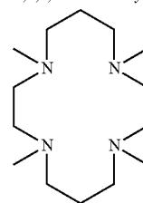
1,4,8,11-tetramethyl-1,4,8,11-tetraazacyclotetradecane
