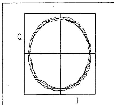
FQPSK-B. VECTOR CONSTELLATION FIG. 19E
