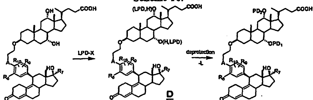
Scheme 10.
