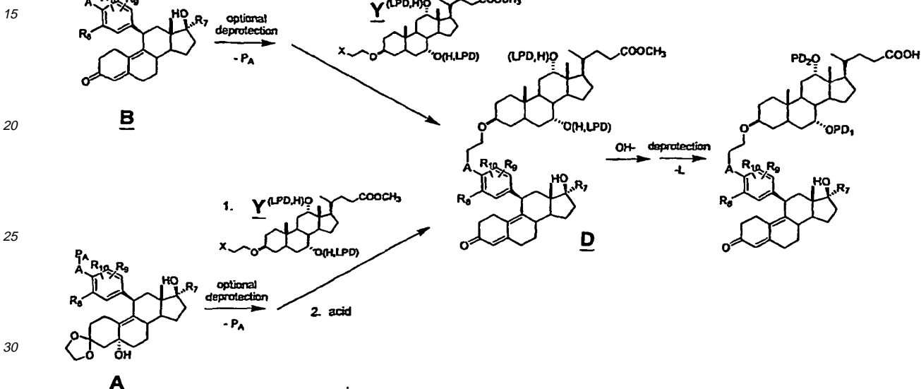
Scheme 8.
