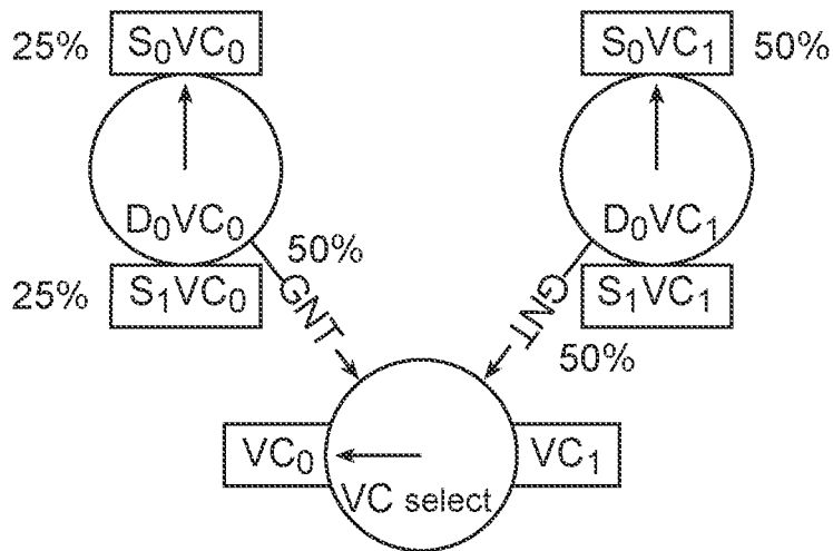
Simple LRU VC select Grant vector:
