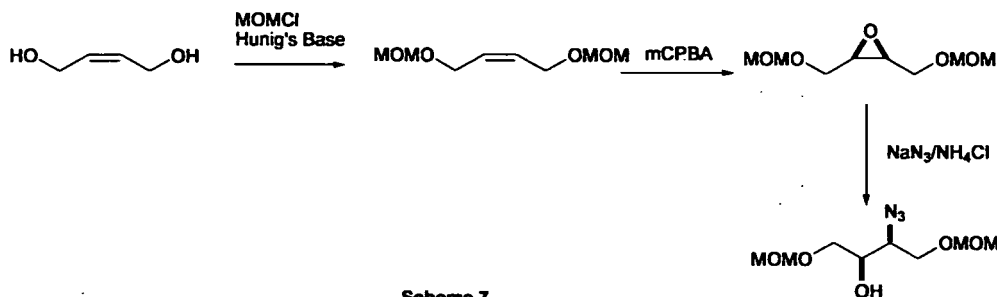
Scheme 7
