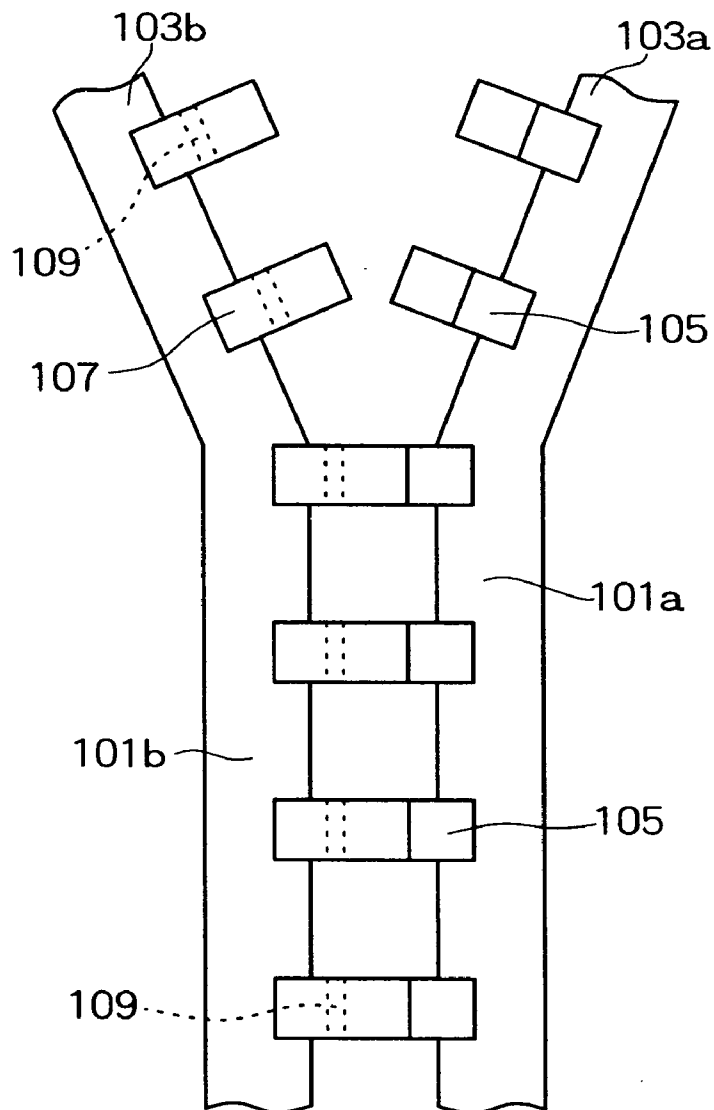
FIG. 9 PRIOR ART
