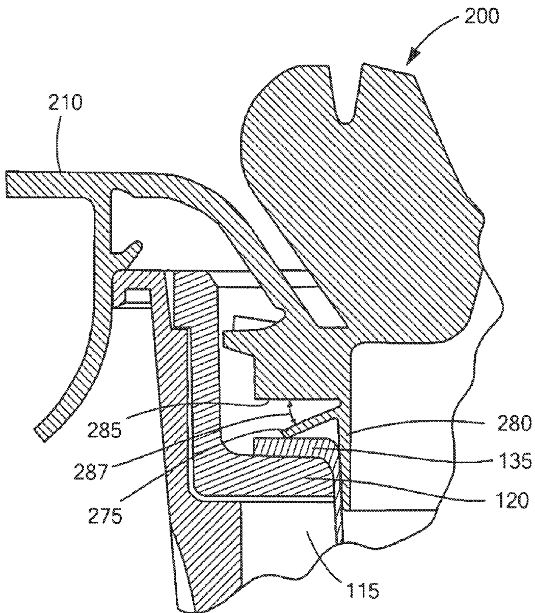
DETAIL K
