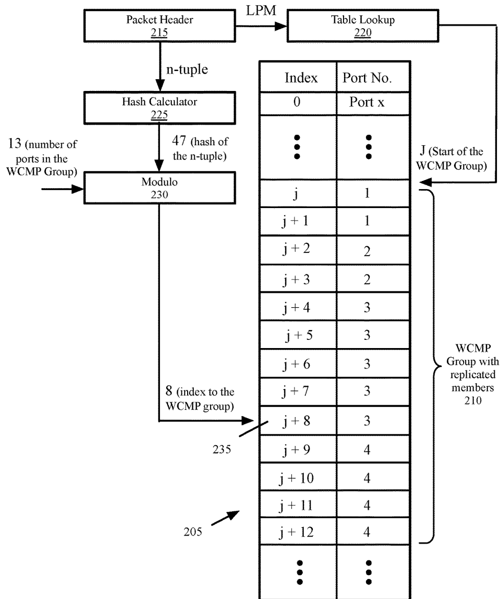
Fig. 2 (Prior Art)
