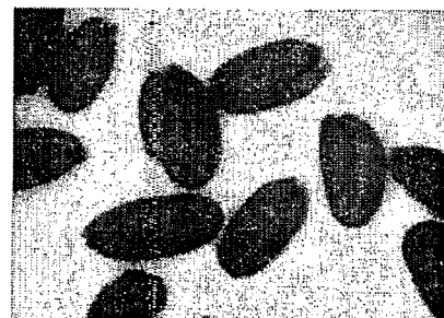
35S::MNT RNAi line 2 mean wt 35.6 \mu g
