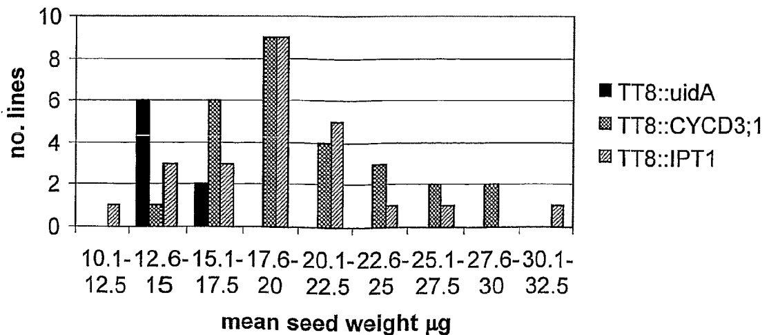
Distribution of seed weights in TT8::uidA (control), TT8::CYCD3;1, and TT8::IPT1 families
