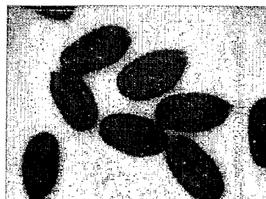
35S::MNT RNAi line 4 mean wt 36.7 \mu g
