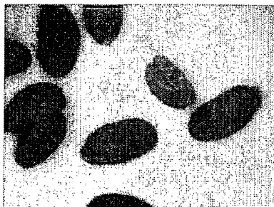
35S::MNT RNAi line 3 mean wt 34.8 \mu g
