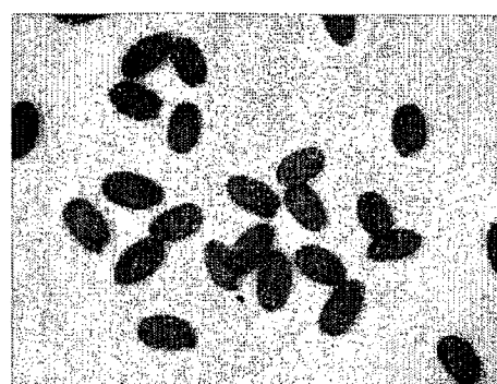
BAN::CYCD3;1 line 1 mean wt 23.9 \mu g
