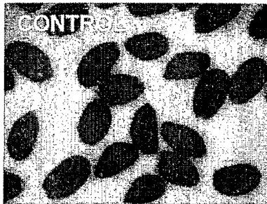
wild-type Col-3 mean wt 13.8 \mu g
