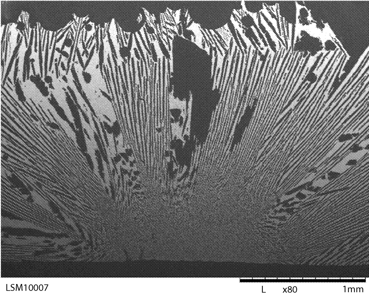
Fired LSM1 cross-section
