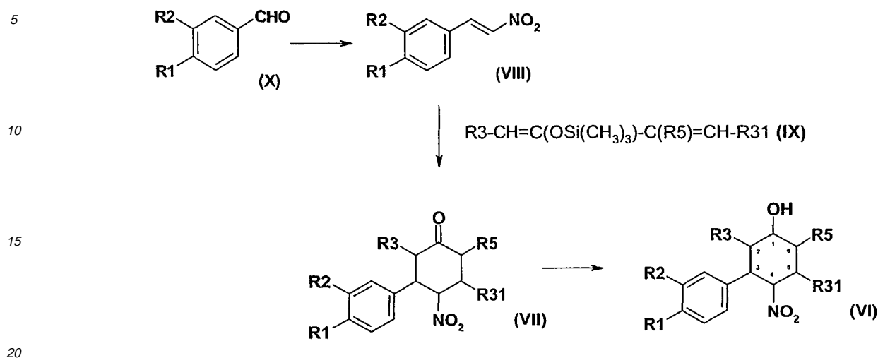
Reaction scheme 2:
