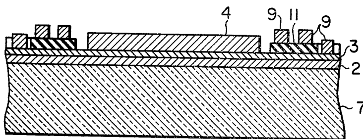
FIG. 3 PRIOR ART
