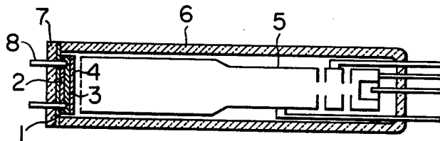
FIG. 1 PRIOR ART
