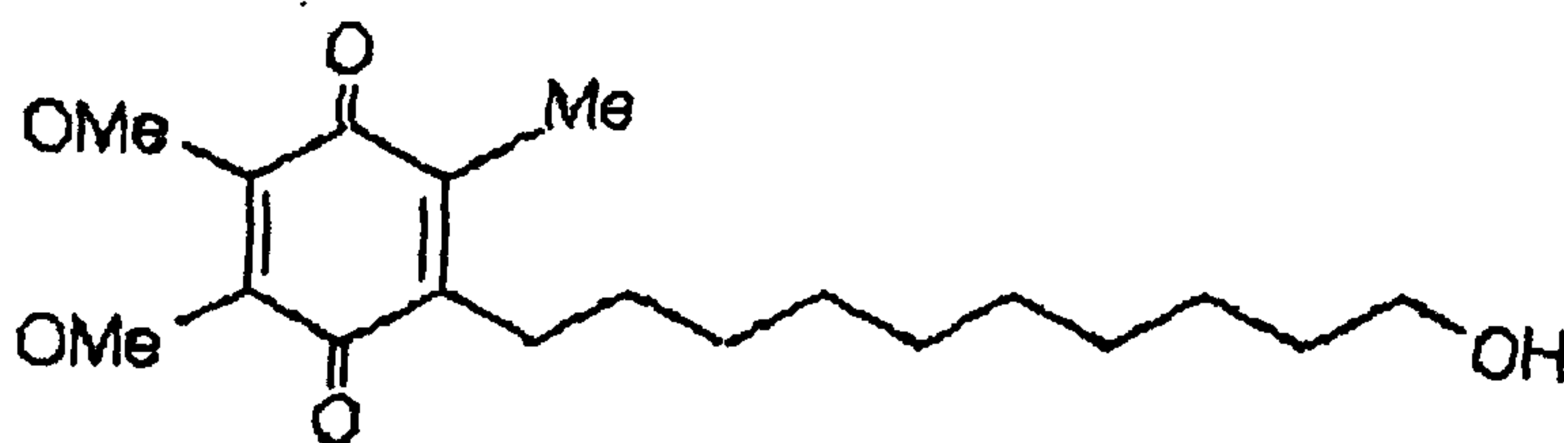
2,3-dimethoxy-5-methyl-6-(10-hydroxydecyl)-1,4-benzoquinone, idebenone
