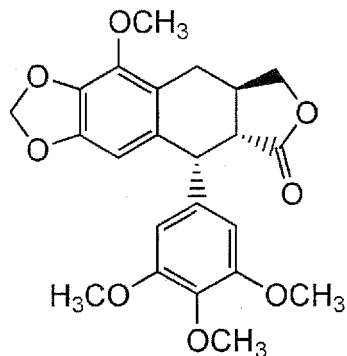
Comparative compound (1)
