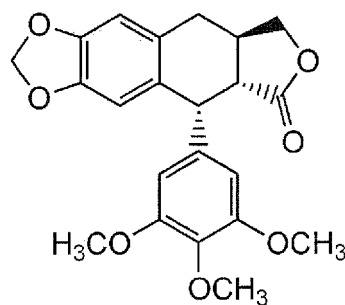
Comparative compound (2)
