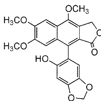
Comparative compound (4)
