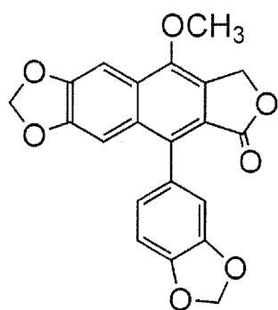
Comparative compound (3)
