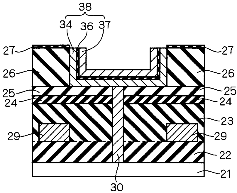
FIG. 11 (BACKGROUND ART)
