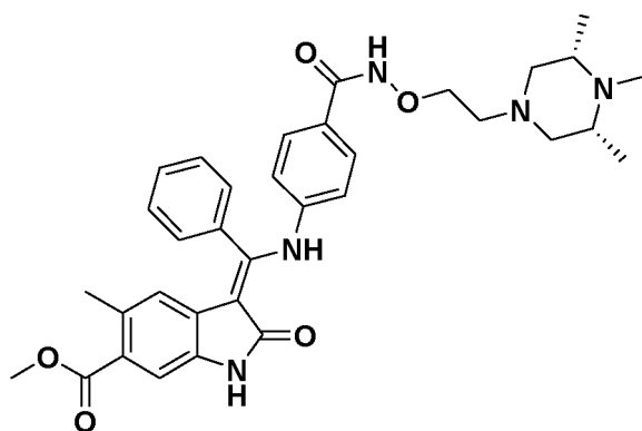
(Z)-Methyl 5-methyl-2-oxo-3-(phenyl((4-((2-((3 R ,5 S )-3,4,5-trimethylpiperazin-1-yl)ethoxy)carbamoyl)phenyl)amino)methylene)indoline-6-carboxylate Route code*: 1C
