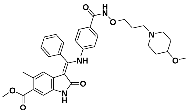
(Z)-Methyl 3-(((4-((3-(4-methoxypiperidin-1-yl)propoxy)carbamoyl)phenyl)amino)(phenyl)methylene)-5-methyl-2-oxoindoline-6-carboxylate Route code*: 1B
