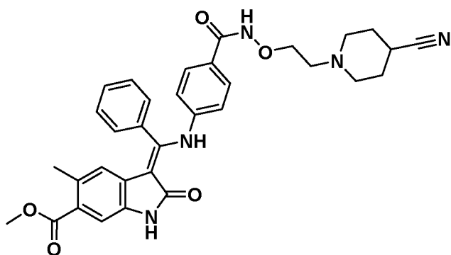
(Z)-Methyl 3-(((4-((2-(4-cyanopiperidin-1-yl)ethoxy)carbamoyl)phenyl)amino)(phenyl)methylene)-5-methyl-2-oxoindoline-6-carboxylate, 0.4 formate Route code*: 1C
