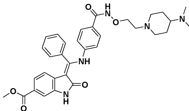
(Z)-Methyl 3-(((4-((2-(4-(dimethylamino)piperidin-1-yl)ethoxy)carbamoyl)phenyl)amino)(phenyl)methylene)-2-oxoindoline-6-carboxylate, formate Route code*: 1C
