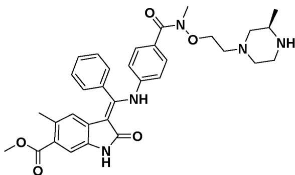
( R,Z )-Methyl 5-methyl-3-(((4-(methyl(2-(3-methylpiperazin-1-yl)ethoxy)carbamoyl)phenyl)amino)(phenyl)methylene)-2-oxoindoline-6-carboxylate Route code*: 1D
