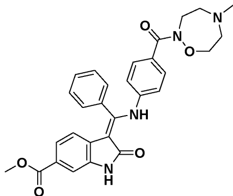
(Z)-Methyl 3-(((4-(5-methyl-1,2,5-oxadiazepane-2-carbonyl)phenyl)amino)(phenyl)methylene)-2-oxoindoline-6-carboxylate
