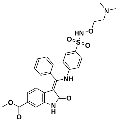
(Z)-Methyl 3-(((4-(N-(2-(dimethylamino)ethoxy)sulfamoyl)phenyl)amino)(phenyl)methylene)-2-oxoindoline-6-carboxylate Route code*: 1A
