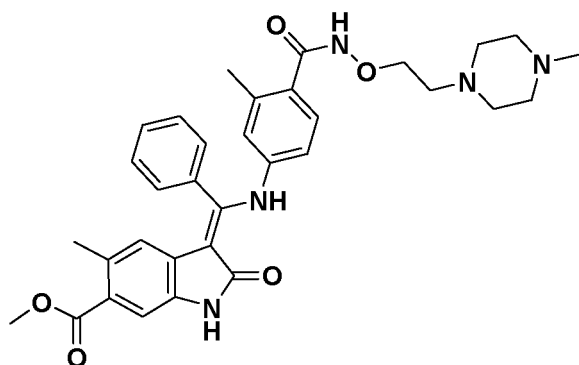
(Z)-Methyl 5-methyl-3-(((3-methyl-4-((2-(4-methylpiperazin-1-yl)ethoxy)carbamoyl)phenyl)amino)(phenyl)methylene)-2-oxoindoline-6-carboxylate
