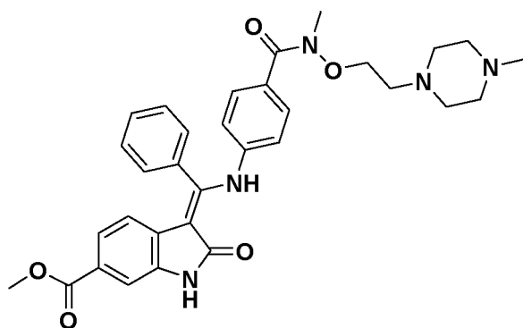
(Z)-Methyl 3-(((4-(methyl(2-(4-methylpiperazin-1-yl)ethoxy)carbamoyl)phenyl)amino)(phenyl)methylene)-2-oxindoline-6-carboxylate Route code*: 1B
