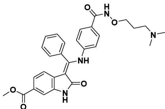
(Z)-Methyl 3-(((4-((3-(dimethylamino)propoxy)carbamoyl)phenyl)amino)(phenyl)methylene)-2-oxoindoline-6-carboxylate
