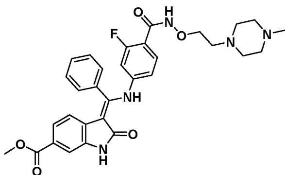
(Z)-Methyl 3-(((3-fluoro-4-((2-(4-methylpiperazin-1-yl)ethoxy)carbamoyl)phenyl)amino)(phenyl)methylene)-2-oxoindoline-6-carboxylate Route code*: 1B
