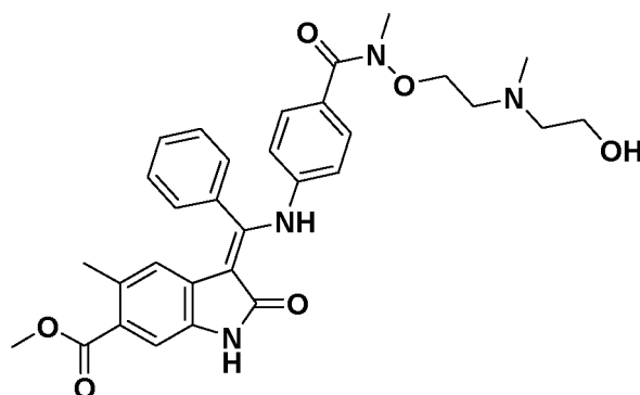
(Z)-Methyl 3-(((4-((2-((2-hydroxyethyl)(methyl)amino)ethoxy)(methyl)carbamoyl)phenyl)amino)(phenyl)methylene)-5-methyl-2-oxoindoline-6-carboxylate Route code*: 1D
