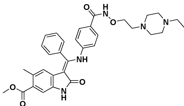
(Z)-Methyl 3-(((4-((2-(4-ethylpiperazin-1-yl)ethoxy)carbamoyl)phenyl)amino)(phenyl)methylene)-5-methyl-2-oxoindoline-6-carboxylate
