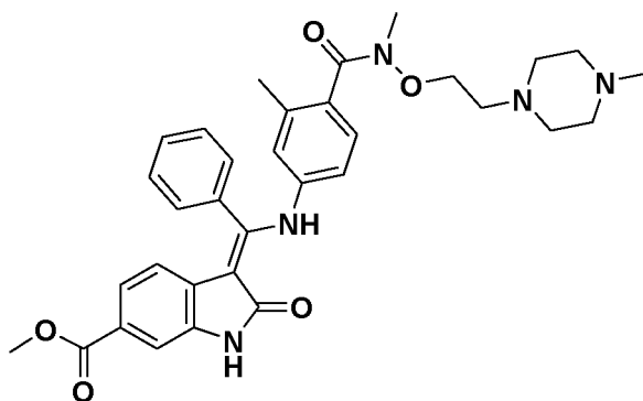
(Z)-Methyl 3-(((3-methyl-4-(methyl(2-(4-methylpiperazin-1-yl)ethoxy)carbamoyl)phenyl)amino)(phenyl)methylene)-2-oxoindoline-6-carboxylate Route code*: 1B
