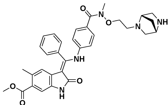
(Z)-Methyl 3-(((4-((2-((1S,4S)-2,5-diazabicyclo[2.2.1]heptan-2-yl)ethoxy)(methyl)carbamoyl)phenyl)amino)(phenyl)methylene)-5-methyl-2-oxoindoline-6-carboxylate Route code*: 1D
