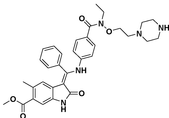
(Z)-Methyl 3-(((4-(ethyl(2-(piperazin-1-yl)ethoxy)carbamoyl)phenyl)amino)(phenyl)methylene)-5-methyl-2-oxoindoline-6-carboxylate Route code*: 1B
