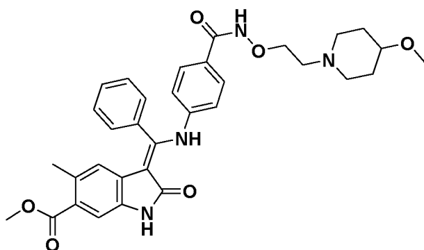
(Z)-Methyl 3-(((4-((2-(4-methoxypiperidin-1-yl)ethoxy)carbamoyl)phenyl)amino)(phenyl)methylene)-5-methyl-2-oxoindoline-6-carboxylate Route code*: 1C
