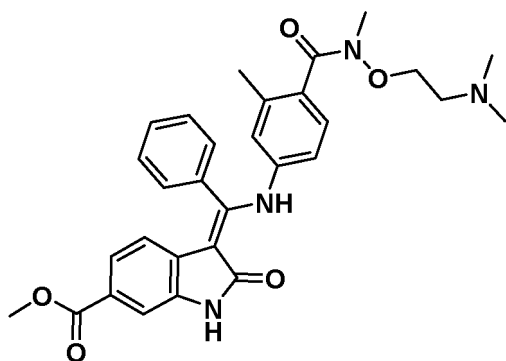
(Z)-Methyl 3-(((4-((2-(dimethylamino)ethoxy)(methyl)carbamoyl)-3-methylphenyl)amino)(phenyl)methylene)-2-oxoindoline-6-carboxylate Route code*: 1B
