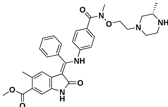
(S,Z)-Methyl 5-methyl-3-(((4-(methyl(2-(3-methylpiperazin-1-yl)ethoxy)carbamoyl)phenyl)amino)(phenyl)methylene)-2-oxoindoline-6-carboxylate Route code*: 1D
