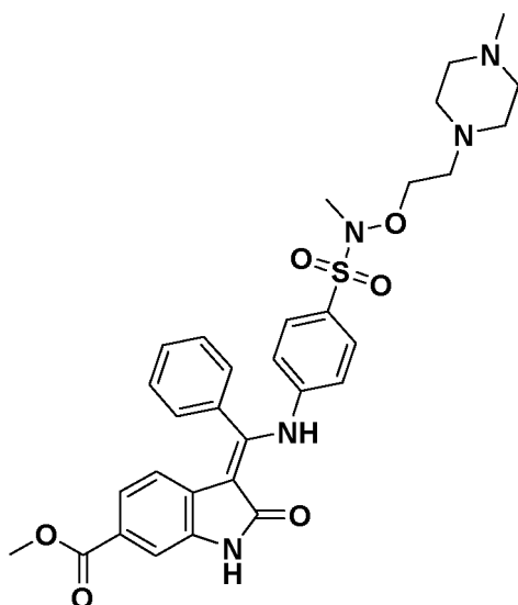
(Z)-Methyl 3-(((4-(N-methyl-N-(2-(4-methylpiperazin-1-yl)ethoxy)sulfonyl)phenyl)amino)(phenyl)methylene)-2-oxoindoline-6-carboxylate
