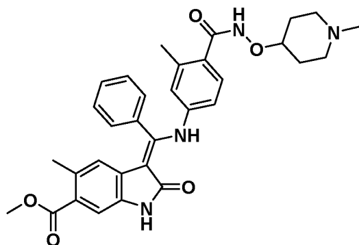
(Z)-Methyl 5-methyl-3-(((3-methyl-4-(((1-methylpiperidin-4-yl)oxy)carbamoyl)phenyl)amino)(phenyl)methylene)-2-oxoindoline-6-carboxylate Route code*: 1B
