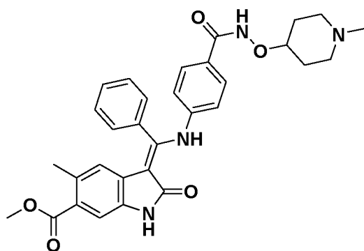
(Z)-Methyl 5-methyl-3-(((4-(((1-methylpiperidin-4-yl)oxy)carbamoyl)phenyl)amino)(phenyl)methylene)-2-oxoindoline-6-carboxylate Route code*: 1B
