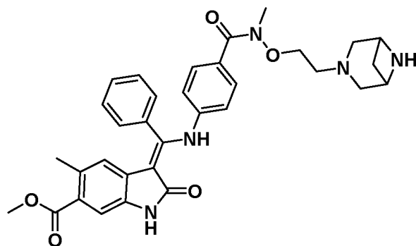
( Z )-Methyl 3-(((4-((2-(3,6-diazabicyclo[3.1.1]heptan-3-yl)ethoxy)(methyl)carbamoyl)phenyl)amino)(phenyl)methylene)-5-methyl-2-oxoindoline-6-carboxylate Route code*: 1D
