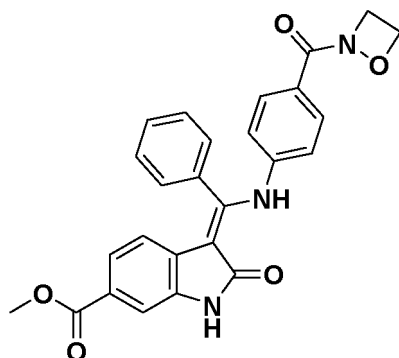
(Z)-Methyl 3-(((4-(1,2-oxazetidine-2-carbonyl)phenyl)amino)(phenyl)methylene)-2-oxoindoline-6-carboxylate
