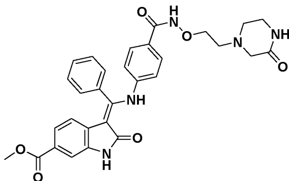
(Z)-Methyl 2-oxo-3-(((4-((2-(3-oxopiperazin-1-yl)ethoxy) carbamoyl)phenyl)amino) (phenyl)methylene)indoline-6-carboxylate Route code*: 1C
