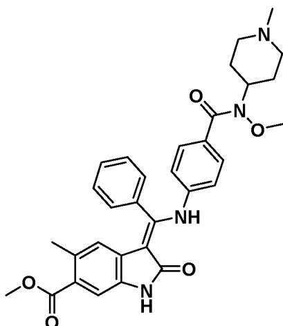
(Z)-Methyl 3-(((4-(methoxy(1-methylpiperidin-4-yl) carbamoyl)phenyl)amino)(phenyl)methylene)-5-methyl-2-oxoindoline-6-carboxylate Route code*: 1B
