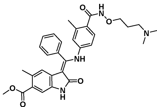
(Z)-Methyl 3-(((4-((3-(dimethylamino)propoxy)carbamoyl)-3-methylphenyl)amino)(phenyl)methylene)-5-methyl-2-oxoindoline-6-carboxylate
