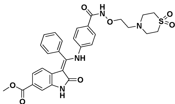
(Z)-Methyl 3-(((4-((2-(1,1-dioxidothiomorpholino)ethoxy) carbamoyl)phenyl)amino) (phenyl)methylene)-2-oxoindoline-6-carboxylate Route code*: 1C
