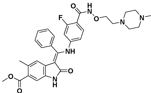
(Z)-Methyl 3-(((3-fluoro-4-((2-(4-methylpiperazin-1-yl)ethoxy)carbamoyl)phenyl)amino)(phenyl)methylene)-5-methyl-2-oxoindoline-6-carboxylate Route code*: 1B
