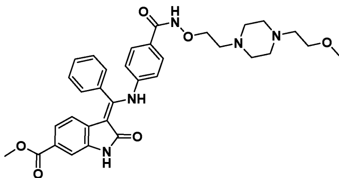
(Z)-Methyl 3-(((4-((2-(4-(2-methoxyethyl)piperazin-1-yl)ethoxy)carbamoyl)phenyl)amino)(phenyl)methylene)-2-oxoindoline-6-carboxylate, formate Route code*: 1C
