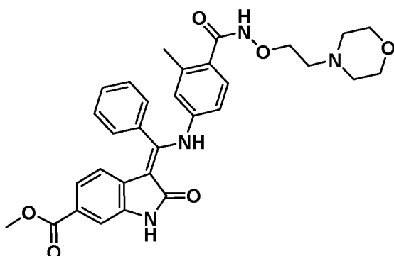
(Z)-Methyl 3-(((3-methyl-4-((2-morpholinoethoxy)carbamoyl)phenyl)amino)(phenyl)methylene)-2-oxoindoline-6-carboxylate Route code*: 1B
