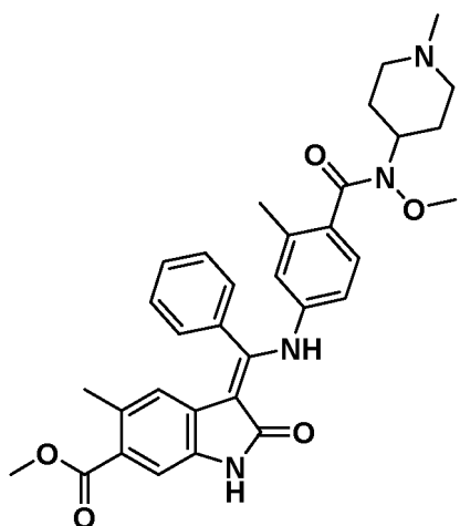
(Z)-Methyl 3-(((4-(methoxy(1-methylpiperidin-4-yl) carbamoyl)-3-methylphenyl)amino)(phenyl)methylene)-5-methyl-2-oxoindoline-6-carboxylate Route code*: 1B
