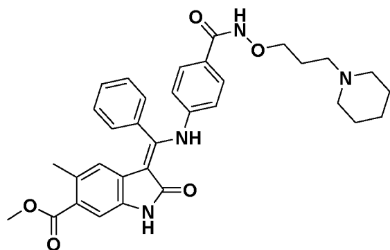
(Z)-Methyl 5-methyl-2-oxo-3-(phenyl((4-((3-(piperidin-1-yl)propoxy)carbamoyl)phenyl)amino)methylene)indolin e-6-carboxylate Route code*: 1B
