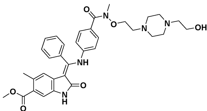
(Z)-Methyl 3-(((4-((2-(4-(2-hydroxyethyl)piperazin-1-yl)ethoxy)(methyl)carbamoyl)phenyl)amino)(phenyl)methylene)-5-methyl-2-oxoindoline-6-carboxylate Route code*: 1D
