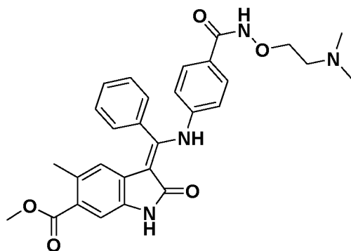
(Z)-Methyl 3-(((4-((2-(dimethylamino)ethoxy)carbamoyl)phenyl)amino)(phenyl)methylene)-5-methyl-2-oxoindoline-6-carboxylate Route code*: 1B
