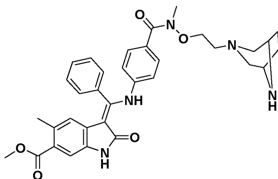
(Z)-Methyl 3-(((4-((2-(3,8-diazabicyclo[3.2.1]octan-3-yl)ethoxy)(methyl)carbamoyl)phenyl)amino)(phenyl)methylene)-5-methyl-2-oxoindoline-6-carboxylate Route code*: 1D
