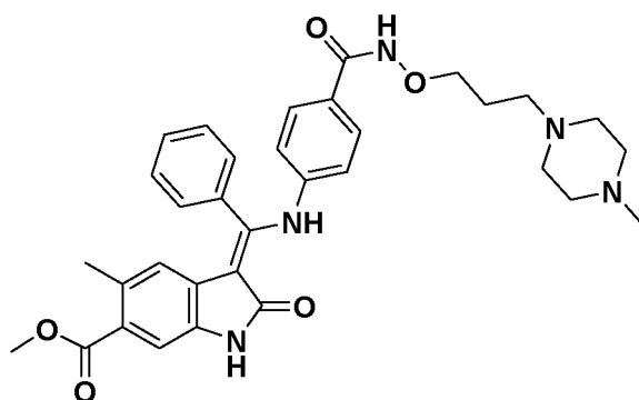
(Z)-Methyl 5-methyl-3-(((4-((3-(4-methylpiperazin-1-yl)propoxy)carbamoyl)phenyl)amino)(phenyl)methylene)-2-oxoindoline-6-carboxylate Route code*: 1B
