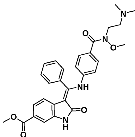
(Z)-Methyl 3-(((4-((2-(dimethylamino)ethyl)(methoxy)carbamoyl)phenyl)amino)(phenyl)methylene)-2-oxoindoline-6-carboxylate Route code*: 1B
