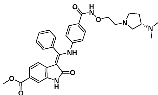
(S,Z)-Methyl 3-(((4-((2-(3-(dimethylamino)pyrrolidin-1-yl)ethoxy)carbamoyl)phenyl)amino)(phenyl)methylene)-2-oxoindoline-6-carboxylate, formate
